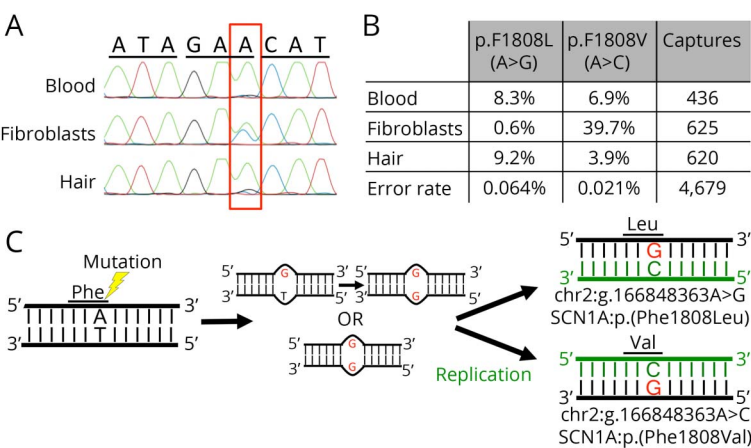
Figure Two SCN1A mosaic variants at the same nucleotide position in an individual with Dravet syndrome
