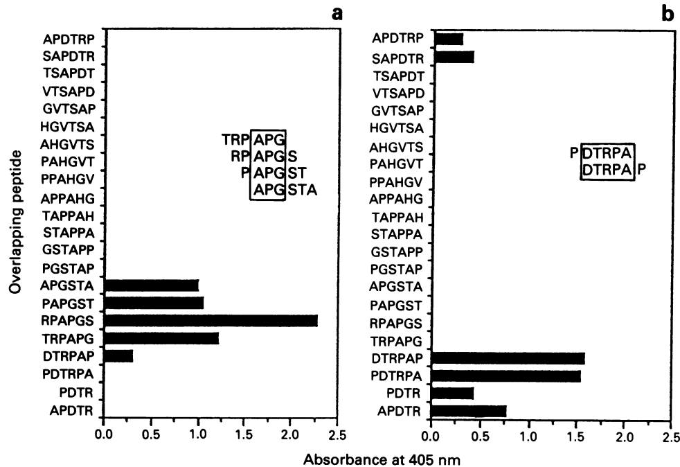
Figure 5 Reactivity of 1/10 dilution of tissue culture supernatant of (a) VA1 and (b) VA2 with synthetic peptides synthesised on pins.
