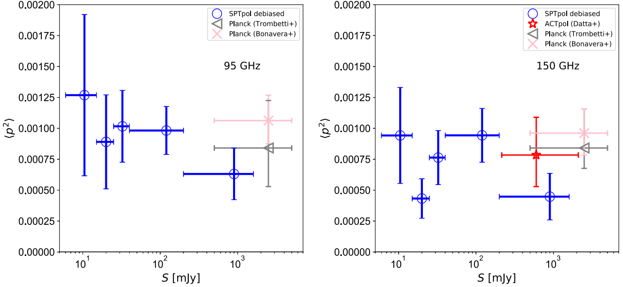
Figure 3. Estimated \langle p^2 \rangle for extragalactic radio sources at 95 (left-hand panel) and 150 GHz (right-hand panel). The blue data points represent de-biased \langle p^2 \rangle values in five flux bins split according to the SPT–SZ 150 GHz flux in both panels. The horizontal bars on data points represent bin size and the vertical error bars are computed using bootstrapping (see Section 3.3). For comparison, we also show the squared values of polarization fraction \langle p \rangle^2 measured by Bonavera et al. (2017a) and Trombetti et al. (2018) both at 100 (left-hand panel) and 143 GHz (right-hand panel) and Datta et al. (2018) (at 148 GHz in the right-hand panel) for high-flux radio sources.
