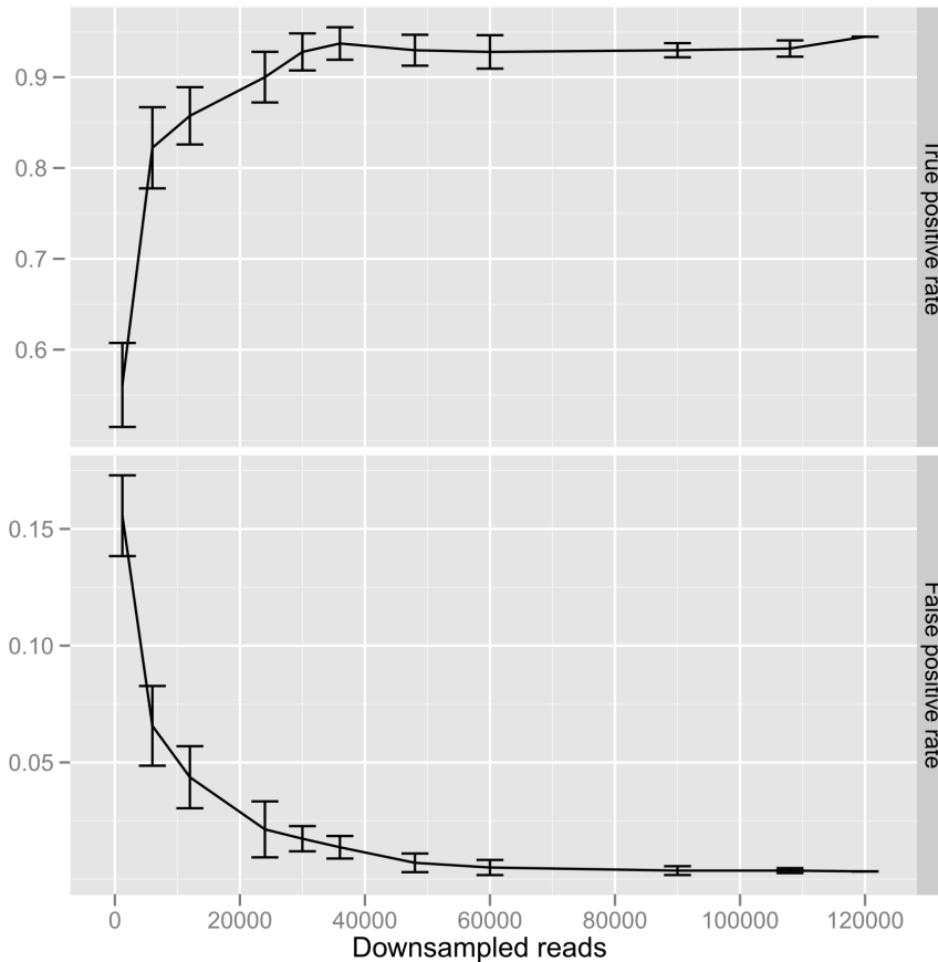
Figure 3. Effect of down-sampling Illumina coverage on true positive and false positive rates. Plots are of the median true positive and false positive minority variant detection rates of the control library with the standard deviation shown as error bars from 10 iterations of random sampling from all reads to generate each coverage depth. doi:10.1371/journal.pone.0090485.g003
