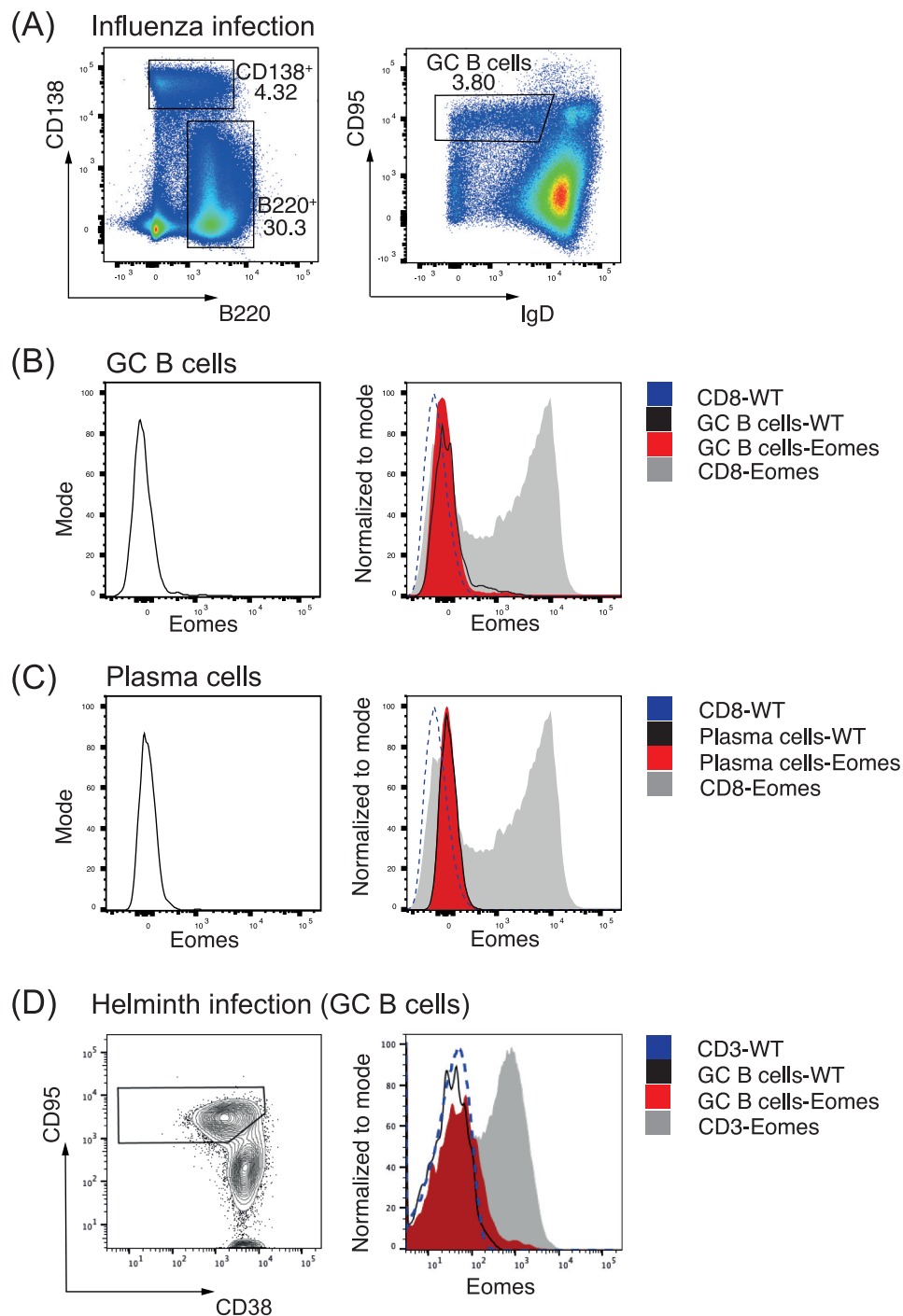
Fig 5. Eomes is not detected in germinal center B cells during either Th1 or Th2 infection. (A-C) Representative flow cytometric plots of influenza-infected Eomes mcherry/+ (reporting for Eomes mRNA transcript) or C57BL/6 mice. Splenic germinal center B cells (A, B), plasma cells (A, C) and CD8 T cells (B-C) were assessed for Eomes expression 8 days post-infection. CD8 T cells from C57BL/6 mice are represented by the dotted line. (D) Representative flow cytometric plots of mice that were infected with T. muris and assessed for Eomes expression in germinal center B cells and CD3 + T cells 21 days post-infection. Eomes mcherry/+ data are representative of \geq 3 mice per experiment.
