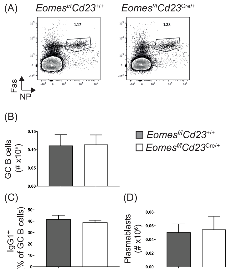
Fig 1. Eomes is not required for B cell differentiation in response to immunization with NP-KLH in alum. Eomes f/f Cd23 Cre/+ and littermate controls were immunized with NP-KLH precipitated in alum. Splenic B cell subsets were assessed at day 14 post-immunization. (A) Representative plots of antigen-specific germinal center B cells (NP + Fas + B cells). Germinal center B cell number (B), the frequency of germinal center B cells that have switched to IgG1 (C) and plasmablast number (D) are shown. Data are pooled from two experiments, n = 5 mice per genotype, and is representative of a third independent experiment. Error bars indicate mean ± SEM. No significant difference was detected using the Mann-Whitney non-parametric test.
