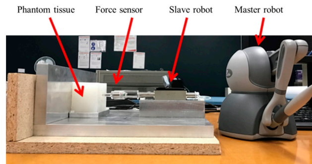
Figure 5. System configuration for robotic indentation.
