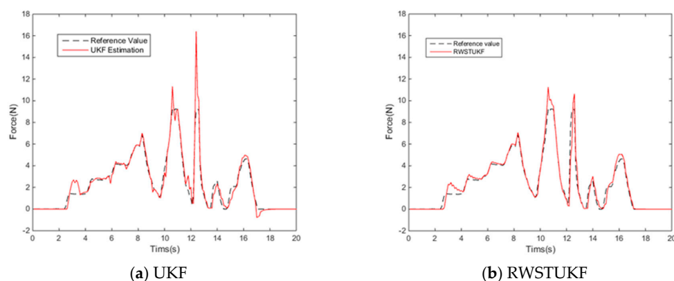
Figure 6. Reconstructed forces via both UKF and RWSTUKF for robotic indentation.
