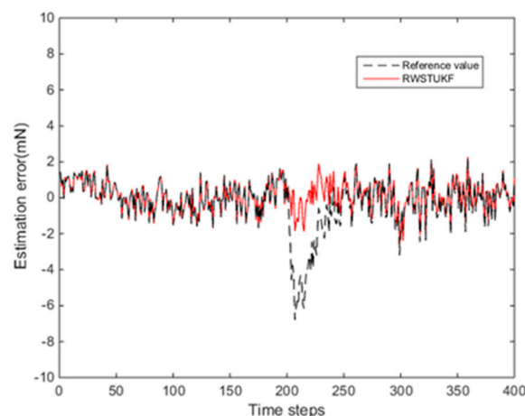
Figure 4. Estimation errors of both UKF and RWSTUKF under local modelling error.
