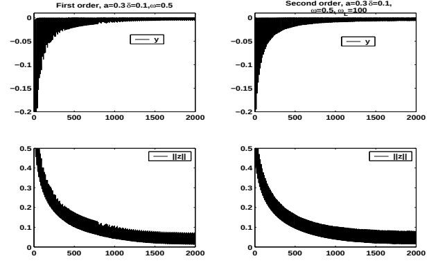
Fig. 8. The comparison between two extremum seeking schemes
