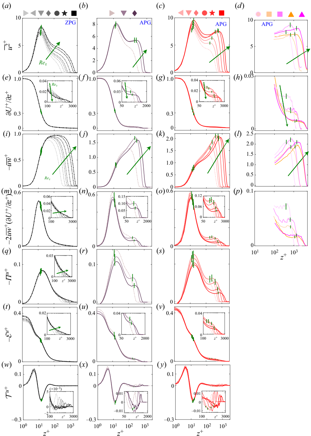
Figure 2. Wall-normal profiles for (a–d) u^2+ , (e–h) \partial U^+/\partial z^+ , (i–l) -\bar{u}w^+ , (m–p) \mathcal{P}^{u+} \approx -2\bar{u}w^+\partial U^+/\partial z^+ , (q–s) -\Pi^{u+} , (t–v) -E^{u+} and (w–y) T^{u+} for ZPG (a,e,i,m,q,t,w) and APG TBL cases (b,f,j,n,r,u,x,c,g,k,o,s,v,y,d,h,l,p). Symbols/colours correspond to the various cases defined in figure 1, with light to dark shading indicating increasing Re_\tau . Note the inconsistent axis ranges.
