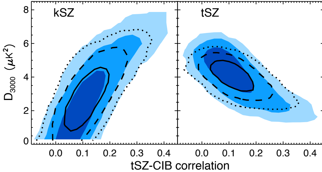
FIG. 6.— The 2d likelihood of the tSZ-CIB correlation and kSZ ( Left panel ) or tSZ power ( Right panel ). The filled contours show the 1, 2, and 3 \sigma constraints. The line contours show the same with the addition of the bispectrum prior on tSZ power. The data strongly prefer a positive correlation, consistent with DSFGs being over-dense in galaxy clusters.
