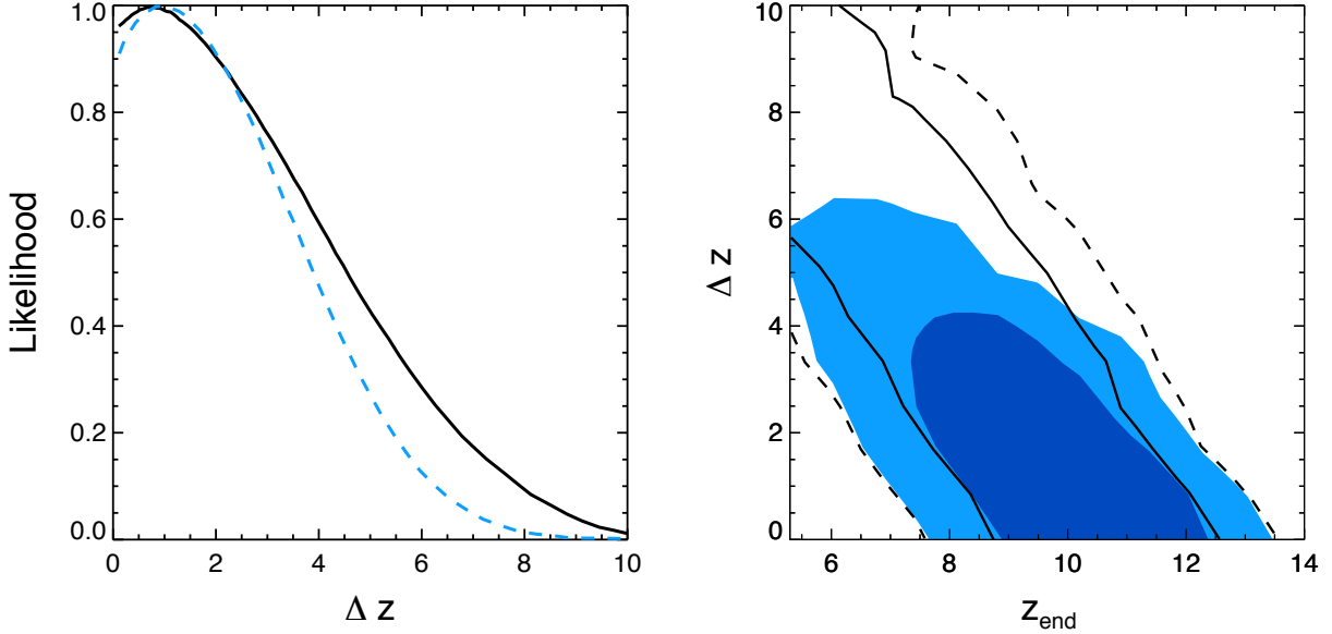
FIG. 10.— Left: 1D likelihood curves for \Delta z of reionization with the homogeneous kSZ fixed to the CSF model. The solid, black line and dashed, blue line lines show the constraint with and without including the bispectrum information. The model including bispectrum constraints leads to the tightest constraint on reionization with an upper limit on the duration \Delta z < 5.4 at 95% CL with the likelihood peaking near \Delta z = 1.3 . Right: The blue, filled contours mark the 1 and 2 \sigma contours of the 2D likelihood surface for \Delta z and z_{\text{end}} ( x_e = 0.99 ), for the fixed CSF model including bispectrum information. Note that the width of the constraint on the z_{\text{end}} axis is primarily set by the errors on the WMAP measurement of \tau . The WMAP only constraint on reionization is shown with the black, solid and dashed contours .
