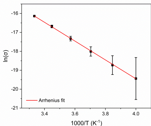
Fig. 4 Arrhenius plot for the [\text{Cu}_2(\text{Me}_2\text{pz})(\text{TCNQ})] compound.
