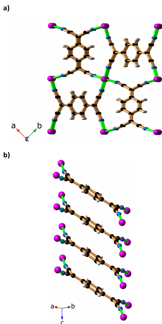
Fig. 6 The structure of \text{Cu(TCNQ)} a) viewed along the c -axis and b) showing a single stack of TCNQ ligands with a side on view; only one orientation of the TCNQ ligands is shown; similarly each Cu centre is disordered over two symmetry-related sites but only half of these sites are indicated in Fig. 6b.
