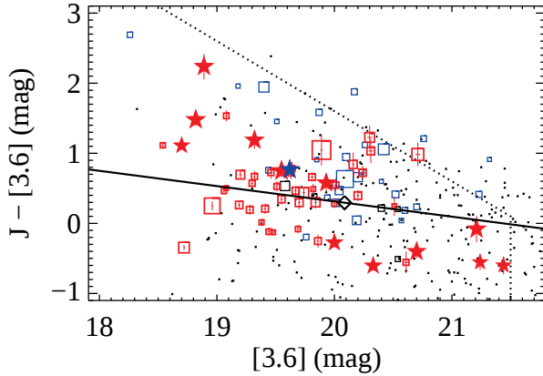
FIG. 2.— Color-magnitude diagram ( J - [3.6] vs. [3.6] ) for galaxies within the IRAC FOV. Suspected red-sequence cluster members are plotted in red. Lower-probability, but potential cluster members are plotted in blue. Spectroscopic members are plotted as stars, where the red stars correspond to passive galaxies and the blue star represents an emission-line galaxy. Additional galaxies in the field are plotted as black points. The size of the symbol is inversely proportional to the distance to the center of the cluster as determined by the clustering of the red-sequence galaxies. Our 5\text{-}\sigma limits are plotted as dotted lines. A red-sequence model corresponding to z = 1.132 is represented as the solid black line with a representative L^* galaxy represented by the black diamond.
