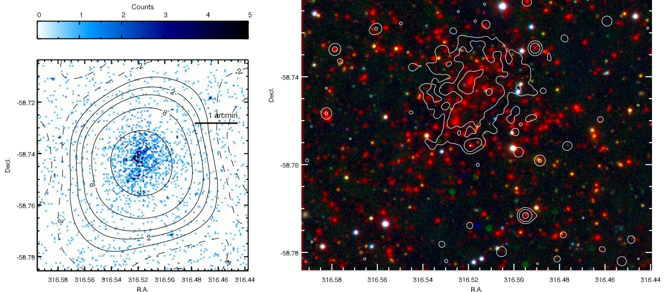
FIG. 4.— SPT-CL J2106-5844 at X-ray, millimeter, optical, and infrared wavelengths. Left: Chandra X-ray image from the 0.7–4.0 keV band, with 4 \times 4 binning of the original ACIS pixels ( 0''.49 on a side). The black contours correspond to the SZ significance from the left-hand panel of Figure 1. Right: LDSS3 optical and Spitzer/IRAC mid-infrared gi[3.6] (corresponding to BRG channels) images. The frame subtends 4'8 \times 4'8 . The white contours are the smoothed X-ray signal from the left panel.
