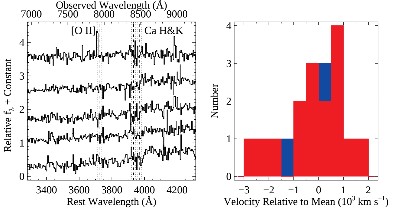
FIG. 3.— Left : Subset of optical spectra of galaxies identified to be cluster members redshifted by the cluster redshift, z = 1.132 . The black vertical dashed lines show the position of [O II] \lambda 3727 and Ca H&K \lambda\lambda 3933, 3968 , while the grey dotted lines show the where the spectral features would fall at \pm 1000 \text{ km s}^{-1} relative to the cluster redshift. Right : Histogram of velocities for the spectroscopic cluster members relative to the biweight mean of all members. The blue and red histograms represent objects with and without obvious [O II] emission, respectively.
