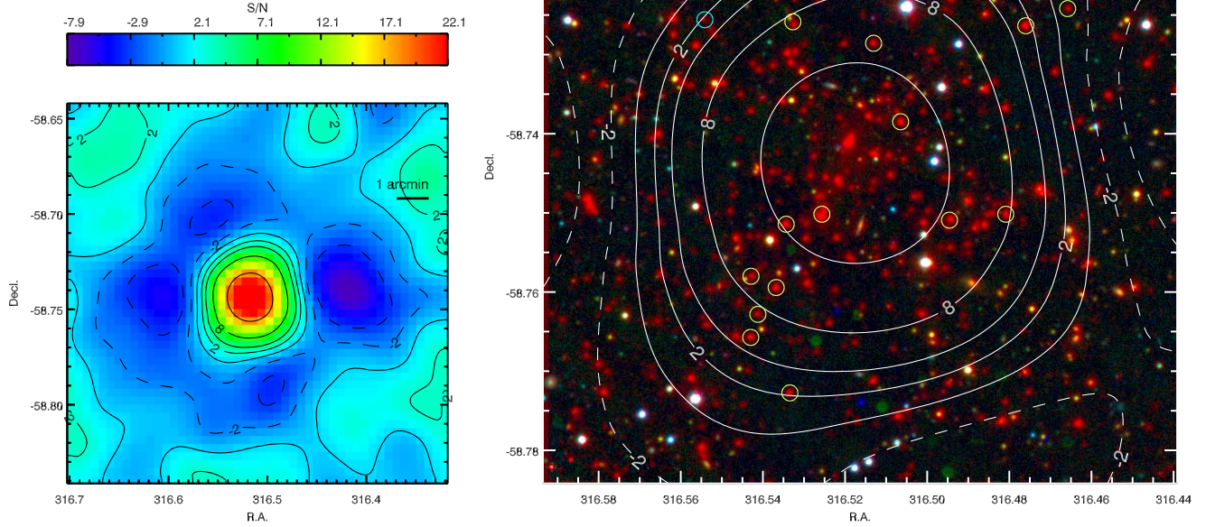
FIG. 1.— SPT-CL J2106-5844 at millimeter, optical, and infrared wavelengths. Left : The filtered SZ significance map derived from multi-band SPT data. The frame subtends 12' \times 12' . The negative trough surrounding the cluster is a result of the filtering of the time ordered data and maps. Right : LDSS3 optical and Spitzer/IRAC mid-infrared gi[3.6] (corresponding to BGR channels) images. The frame subtends 4'8 \times 4'8 . The white contours correspond to the SZ significance from the left-hand panel. The circles mark spectroscopically confirmed cluster members, where green indicates quiescent, absorption-line member galaxies and cyan indicates an active, emission-line member galaxy. Some spectroscopic member galaxies are outside the FOV for this image.
