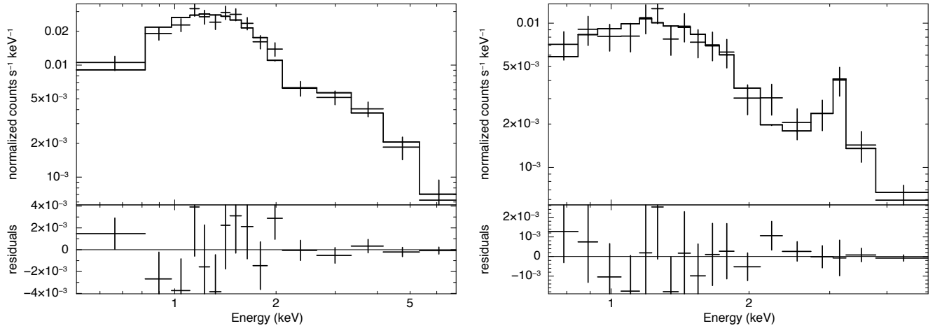
FIG. 5.— Core-excluded (circular annulus spanning 0.15\text{--}1\ r_{500} ) and central region (circular aperture with radius 0.17\ r_{500} ) X-ray spectra of SPT-CL J2106-5844 (left and right panels, respectively). Overplotted (solid line) is a fit APEC spectrum redshifted to z = 1.18 and folded through the detector sensitivity. The 6.7\text{ keV} Fe K line observed at \sim 3\text{ keV} is both obvious and strong for the spectrum from the central region.
