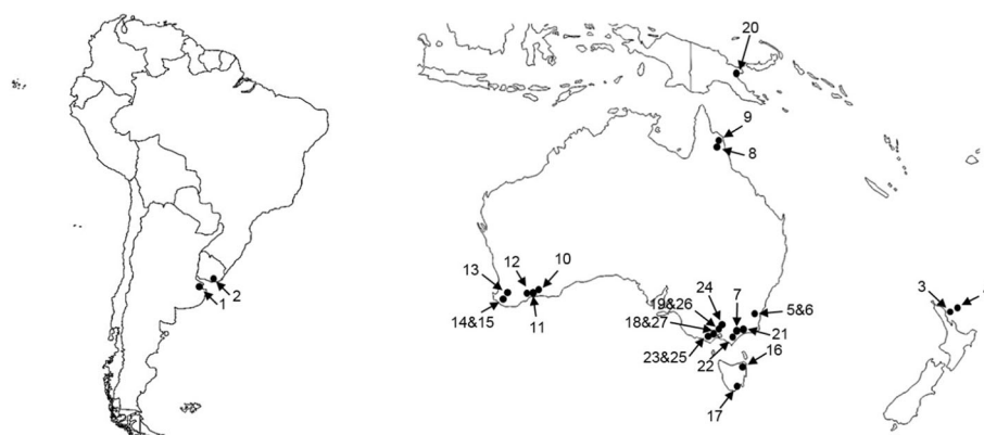
Fig. 1 Collection sites for Ixodes species from Argentina, Australia, New Zealand and Uruguay, used in this study. Information linked to each unique number on the map is provided in Table 1
