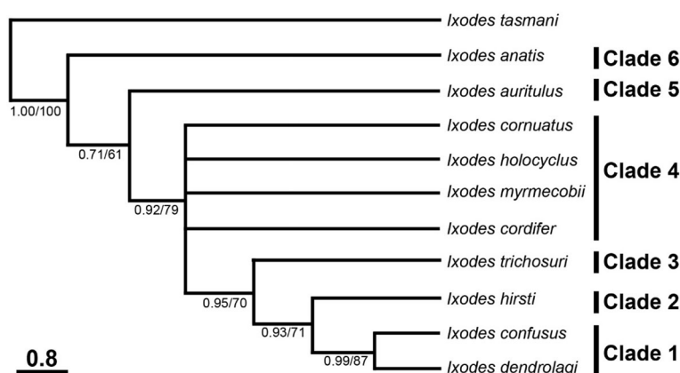
Fig. 3 Morphological phylogram of specimens of Sternalixodes from Argentina, Australia, New Zealand and Uruguay. The relationships were inferred based on 38 morphological characters using Maximum Parsimony (MP) and Bayesian Inference (BI) methods. Ixodes tasmani was used as the outgroup. There was a concordance in the topology between this MP tree and that produced using BI (not shown). Nodal support (from left to right) is given as a posterior probability for BI and bootstrap values for MP. For simplicity, each clade number includes taxa in the preceding clade. The scale-bar indicates the number of inferred substitutions per character
