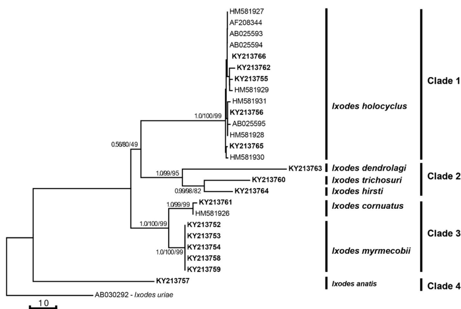
Fig. 5 Genetic relationships of specimens of Sternalixodes from Argentina, Australia, New Zealand and Uruguay. The relationships were inferred based on phylogenetic analyses of the second internal transcribed spacer (ITS-2) sequence data determined herein ( bold ) using Bayesian Inference (BI), distance-based Neighbor Joining (NJ) and Maximum Likelihood (ML) methods. Previously published sequences of Ixodes species were obtained from GenBank (see accession numbers). Ixodes uriae was used as the outgroup. There was a concordance in the topology between this NJ tree and those produced using BI and ML (not shown). Nodal support (from left to right) is given as a posterior probability for BI and bootstrap values for NJ and ML. The scale-bar indicates the number of inferred substitutions per nucleotide site
