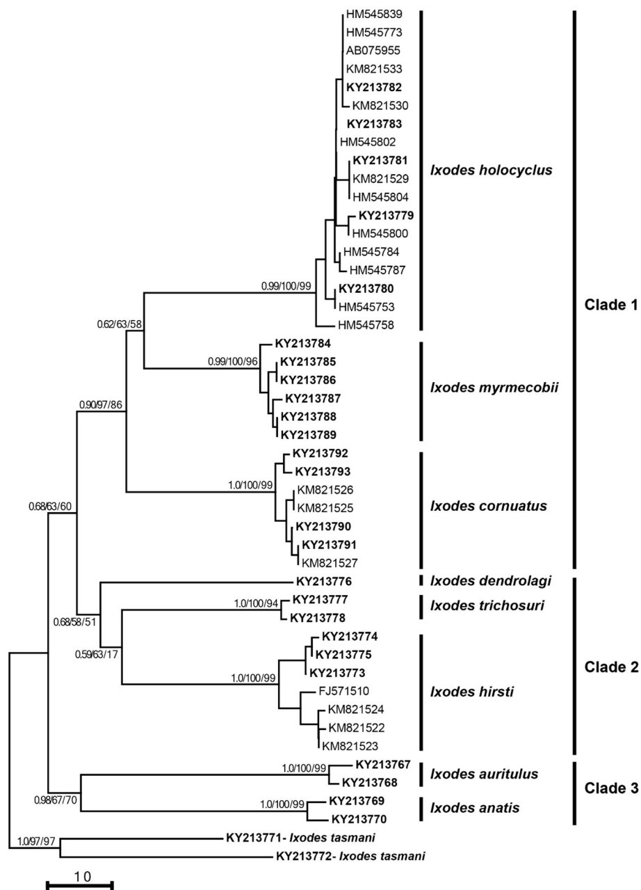
Fig. 4 Genetic relationships of specimens of Sternalixodes from Argentina, Australia, New Zealand and Uruguay. The relationships were inferred based on phylogenetic analyses of the cytochrome c oxidase subunit 1 ( cox1 ) sequence data determined herein ( bold ) using Bayesian Inference (BI), distance-based Neighbor Joining (NJ) and Maximum Likelihood (ML) methods. Previously published sequences of Ixodes species were obtained from GenBank (see accession numbers). Ixodes tasmani was used as the outgroup. There was a concordance in the topology between this NJ tree and those produced using BI and ML (not shown). Nodal support (from left to right) is given as a posterior probability for BI and bootstrap values for NJ and ML. The scale-bar indicates the number of inferred substitutions per nucleotide site
