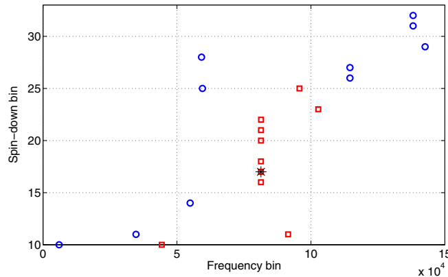
FIG. 6 (color online). Distribution in the frequency/spin-down plane of the top ten candidates obtained in the actual analysis (blue circles) and obtained after the addition to the data of a simulated signal with amplitude h_0 = 4.06 \times 10^{-25} , such that the resulting loudest candidate is approximately as loud as the one obtained in the actual analysis (red squares). The black star identifies the injection. Frequency and spin-down are expressed as the number of bins from the beginning of the corresponding intervals. Six red squares appear to be at the same frequency, but this is just a visual effect due to the large range of frequencies covered by the x axis. In fact, they are very near but spread around the injection values.
