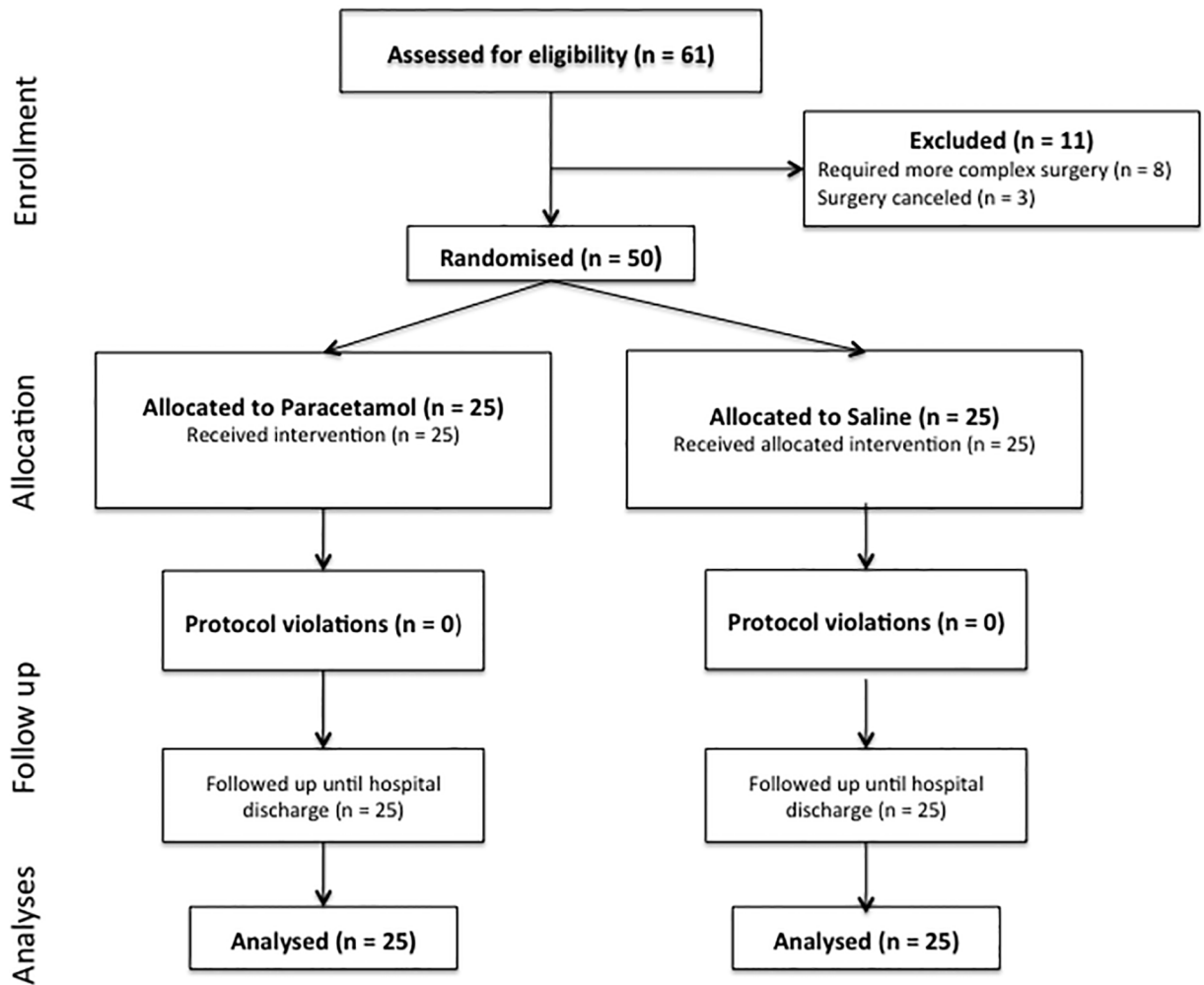
Fig 1. Consort diagram.
