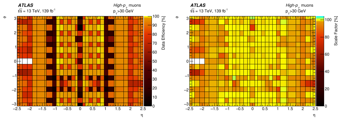
Fig. 15 Reconstruction and identification efficiency measured in collision data (left), and the data/MC efficiency scale factor (right) for High- p_T muons as a function of \eta and \phi for muons with p_T > 30 GeV
