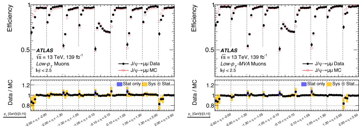
Fig. 16 Muon reconstruction and identification efficiency measured in J/\psi \rightarrow \mu\mu events for the cut-based (left) and multivariate (right) Low- p_T criteria. In the plots, within each \eta region, the efficiency is measured in nine p_T bins (3–3.5, 3.5–4, 4–5, 5–6, 6–7, 7–8, 8–10, 10–12, 12–15 GeV). The resulting values are plotted as distinct measurements in
