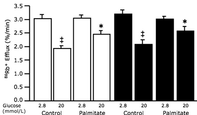
FIG. 4. Potassium efflux in response to 20 mmol/L glucose stimulation is similarly elevated in C57BL/6 and neprilysin-deficient islets after palmitate exposure. Rubidium efflux, reflecting K + permeability, in response to 2.8 and 20 mmol/L glucose stimulation from C57BL/6 and C57BL/6.NEP -/- islets after 48-h culture in the absence or presence of 1 mmol/L palmitate. White bars, C57BL/6 islets; black bars, C57BL/6.NEP -/- islets. Data are means \pm SEM; n = 5 . * P < 0.05 vs. control; ‡ P < 0.001 vs. 2.8 mmol/L glucose.
