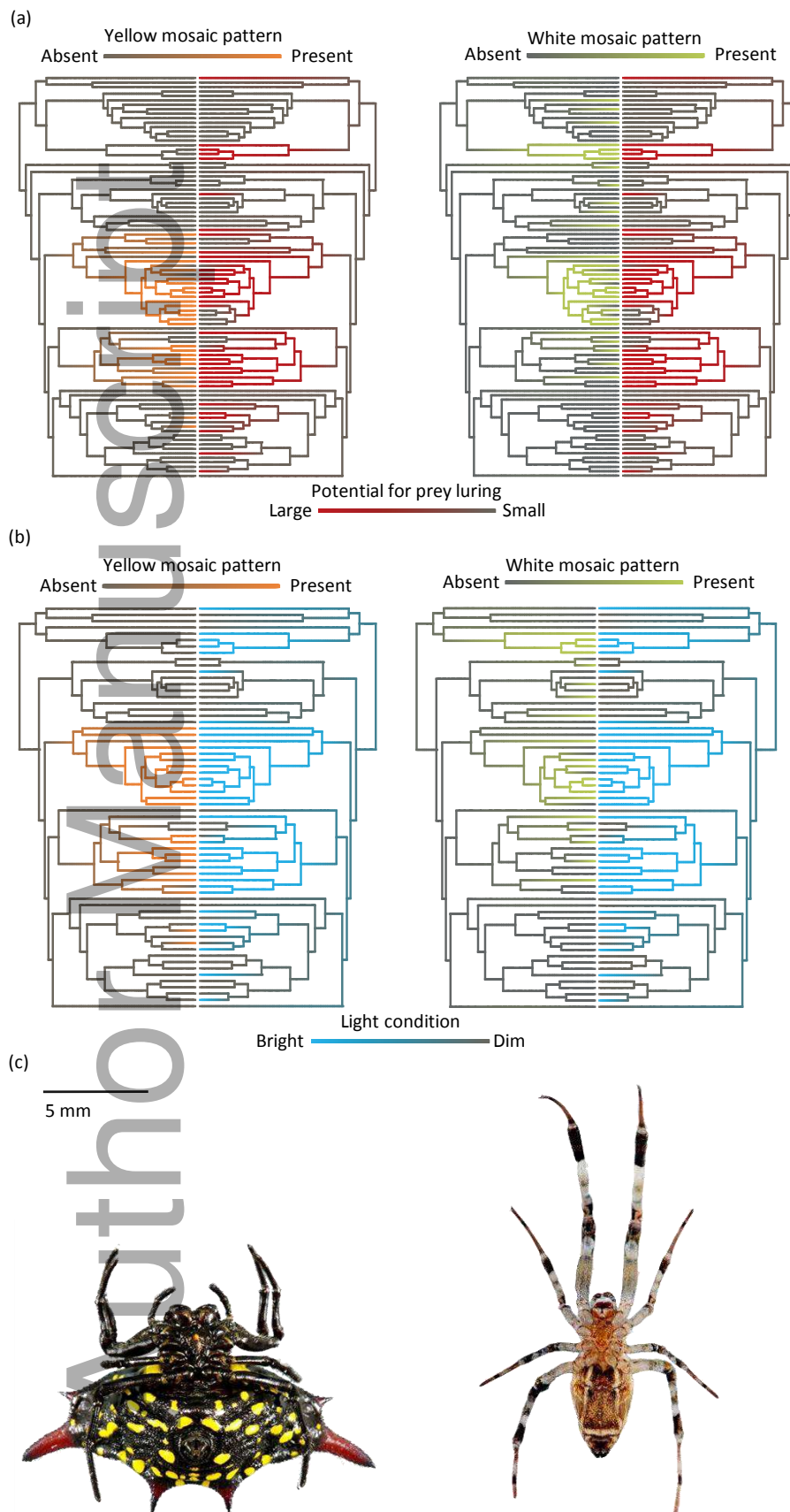
Figure 4. The araneid genus-level phylogeny (derived from Dimitrov et al. (2017)) with colour This article is protected by copyright. All rights reserved
