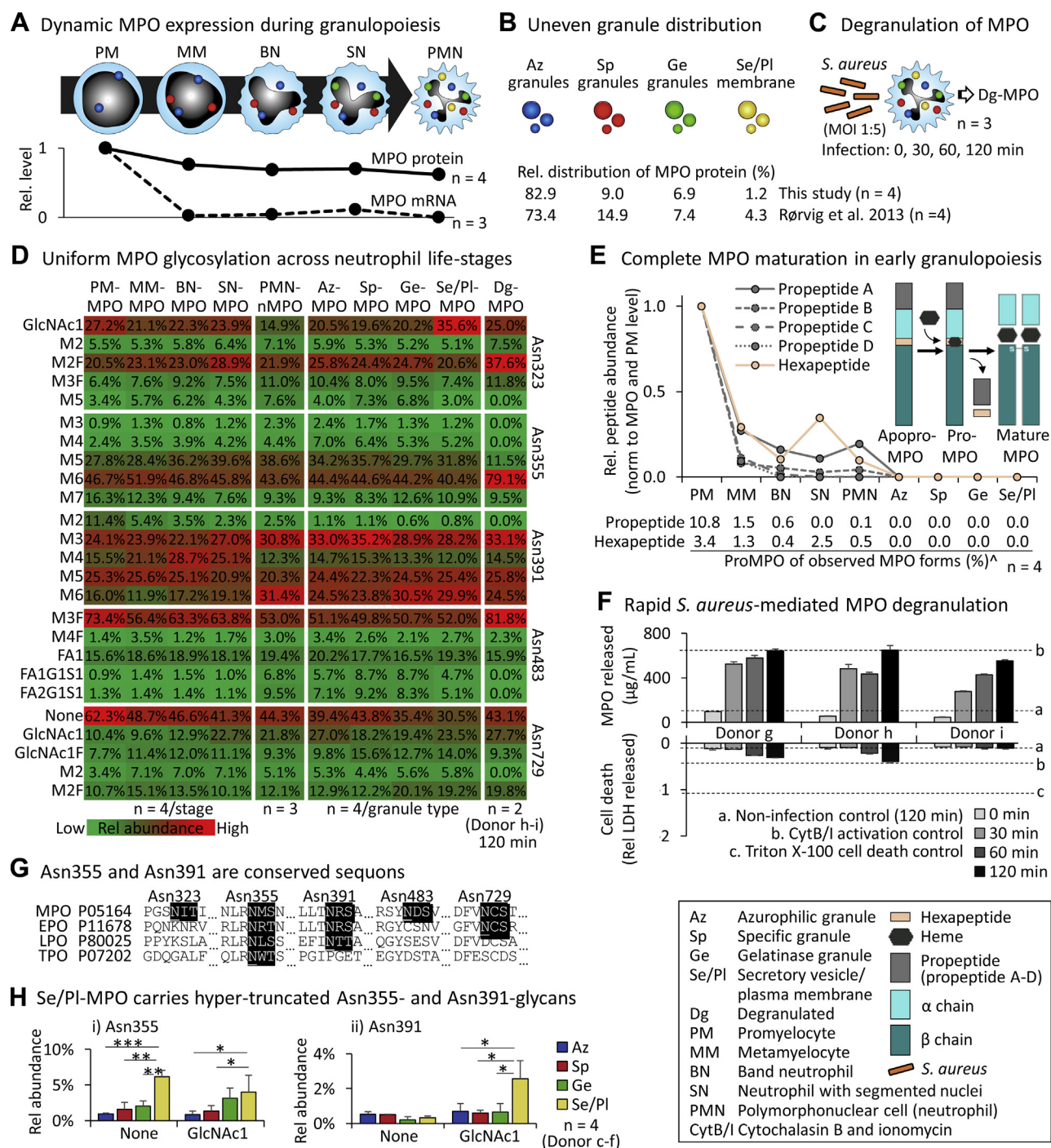
Figure 3. Dynamics, granule distribution, polypeptide processing, site-specific glycosylation and degranulation of MPO across the neutrophil life stages. A , dynamic expression of MPO mRNA ( n = 3 , biological replicates) and protein ( n = 4 , biological replicates) during granulopoiesis. The relative MPO expression levels, normalised to the PM-stage, were established by data re-interrogation (50). See key for nomenclature. B , quantitative proteomics of granule-separated neutrophils ( n = 4 , biological replicates) showed an uneven MPO distribution across granules congruent with literature (18). C , S. aureus -mediated neutrophil activation. Longitudinal profiling of the levels and glycosylation of released Dg-MPO (see panel F , D for data and controls). D , site-specific glycoproteomics of MPO from maturing, resting (PMN-nMPO, see Fig. 1D), granule-separated, and activated neutrophils (average of n = 2-4 plotted, number of biological replicates is indicated). Prominent N-glycans at each site were plotted (Fig. S5 and Table S6). The MPO glycosylation of maturing neutrophils was determined by data re-interrogation (50). See key for intensity scale and biological replicates and Figure 1 for short-hand nomenclature of glycans. E , longitudinal tracking of the proMPO-to-MPO conversion within maturing, mature, and granule-separated neutrophils. Relative levels of peptides arising from the proMPO regions (normalised to PM-stage) were plotted. -ProMPO levels were determined from the intensity of peptide pairs arising from proMPO and mature MPO. The data do not discriminate apoproMPO and proMPO. See insert for schematics of MPO polypeptide maturation (average of n = 4 , biological replicates). F , S. aureus -mediated activation of neutrophils (MOI 1:5) demonstrating a rapid time-dependent and cell death-independent degranulation of Dg-MPO as measured by ELISA and LDH release assays. Controls (a-c, mean plotted as broken lines) were included for both assays ( n = 3 , technical replicates). G , sequence alignment showed that Asn355 and Asn391 are conserved sequons across the human peroxidases implying functional importance. See Figure S6 for sequence alignment to mammalian MPO. H , hyper-truncated GlcNAc \beta Asn and absent glycosylation were elevated features at (i) Asn355 and (ii) Asn391 of Se/PI-MPO relative to MPO from other granules ( n = 4 , biological replicates). For all panels, data plotted as mean \pm SD. ns, not significant ( p \geq 0.05 ), * p < 0.05 , ** p < 0.01 , *** p < 0.005 , **** p < 0.001 , ***** p < 0.00005 . EPO, eosinophil peroxidase; LPO, lactoperoxidase; TPO, thyroid peroxidase.
