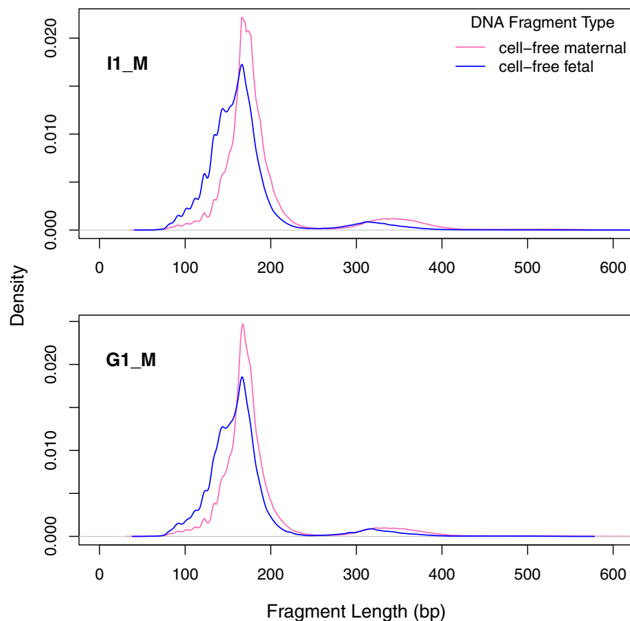
Fig. 8 Size distributions of maternal cell-free DNA contrasted with fetal DNA for two subjects (I1_M and G1_M). Fragments are classed into the two components using allelic information at informative SNPs. Fragment sizes are calculated using the paired-positioning of sequencing reads
