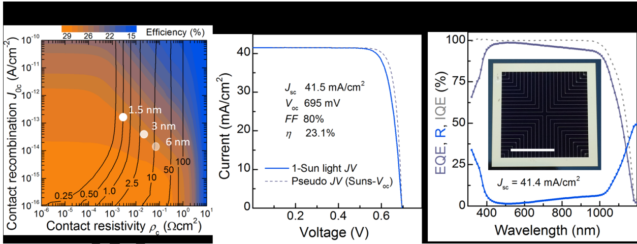
Figure 4: a , simulated ideal efficiency (coloured contours) for a silicon solar cell as a function of the rear contact \rho_c and J_{0c} . For each combination, an ideal contact fraction is also simulated (black lines). The white data points are representative of potential TiO x / LiF x / Al heterocontacts, with different TiO x thicknesses indicated, using information in Figure 1. b , measured light JV characteristics of n-type PRC cell collected under standard 1-Sun conditions (solid line) compared the pseudo JV curve for the same cell measured by Suns- V_{oc} (dashed line). c , quantum efficiency (QE) analysis showing the wavelength dependent external QE, internal QE and reflection. The inset provides a photograph of the cell front design and the integrated short circuit current is also listed. The white scale bar represents 1 cm.
