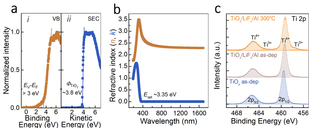
Figure 3: a , measured valence band ( i ) and secondary electron cut-off ( ii ) spectrum of the as-deposited \text{TiO}_x film. b , Tauc-Lorentz modelled refractive index of the as-deposited \text{TiO}_x film showing an optical bandgap of \sim 3.35 eV. c , measured Ti 2p core level spectrum of \text{TiO}_x films after deposition (bottom), capping with a \text{LiF}_x / \text{Al} (middle) and subsequent annealing at 300^\circ\text{C} (top). The \text{LiF}_x / \text{Al} layers were removed via a wet chemical etch prior to measurement for the middle and top samples. The shaded region represents the modelled contribution from different oxidation states to the measured spectrum.
