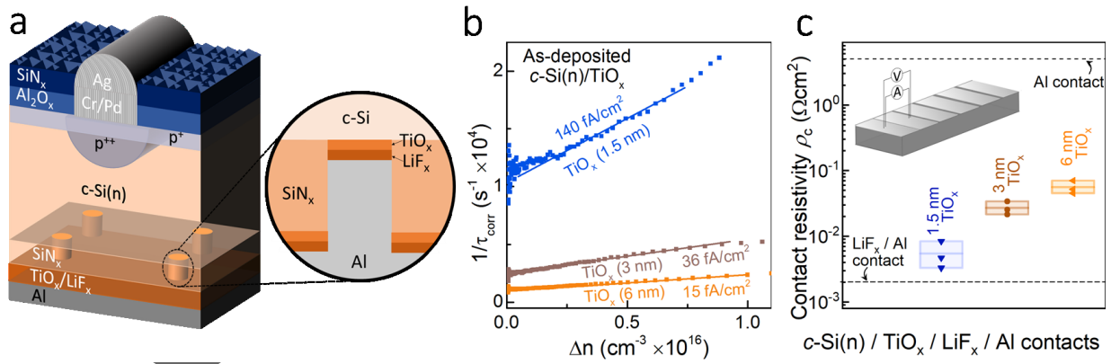
Figure 1: a , conceptual schematic of an n-type PRC cell, the right panel shows a zoom-in of the PRC interface. b , Auger corrected inverse carrier lifetime 1/\tau_{\text{corr}} versus excess carrier density \Delta n used for J_{0c} extraction of three \text{TiO}_x passivated silicon wafers (n-type 1 \Omega\text{cm} ) with different thicknesses of \text{TiO}_x . The extracted J_{0c} values are listed beside each dataset c , extracted \rho_c of three different \text{TiO}_x / \text{LiF}_x / Al heterocontacts on silicon wafers (n-type 1 \Omega\text{cm} ). Three separate samples are measured for each thickness shown by the solid points. The dotted black lines provide a reference for typical \text{LiF}_x / Al and Al contacts and the inset shows a schematic of the TLM structure used in the \rho_c extraction.
