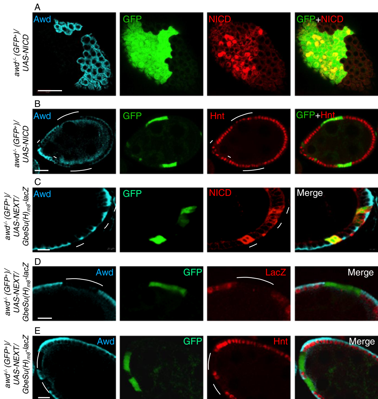
Figure 4 Notch signaling defect in awd mutant cells is rescued by exogenous NICD. Stage 7–8 egg chambers were dissected from females of the genotype hs-flip/GbeSu(H) m8 -lacZ ; act-Gal4 , UAS-GFP/UAS-NICD ; FRT 62B , act-Gal80/FRT 62B , awd 2A4 ( A–B ) or hs-flip/GbeSu(H) m8 -lacZ ; act-Gal4 , UAS-GFP/UAS-NEXT ; FRT 62B , act-Gal80/FRT 62B , awd 2A4 ( C–E ). ( A , C ) As controls, NICD and NEXT expression is verified. ( B ) A stage 7 egg chamber with MARCM clones of awd ( Awd -negative and GFP + , marked by lines) simultaneously expressing NICD. The expression of endogenous Hnt (red) is restored in a majority of the mutant cells. The Awd staining is in cyan. Note that the diffused Awd staining in regions abutting the apical side of the follicle cells is within the germline cells, occasionally observed in abnormal egg chambers. ( D–E ) Exogenously expressed NEXT cannot rescue the awd mutant phenotype. awd MARCM mutant clones lacking Awd staining (cyan) marked by the GFP expression and indicated by lines show loss of GbeSu(H) m8 -lacZ reporter gene expression (red in D ) as well as loss of Hindsight ( Hnt ) expression (red in E ). Bars in ( A–B ) are 20 \mu m. Bars in ( C–E ) are 10 \mu m. NEXT, Notch external truncation; NICD, Notch intracellular domain.
