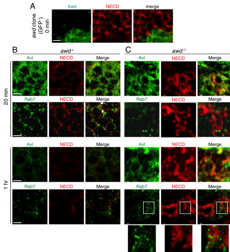
Figure 7 Endocytic defects in awd mutant cells. Notch trafficking assay was performed on wing discs from (A, C) yw; en2.4-Gal4 UAS /+, Ubi-GFP, FRT 82B /FRT 82B , awd Δ2A4 and (B) yw third-instar larvae. (A) In a disc containing awd mutant clone (GFP-negative cells) without synchronized induction of endocytosis (steady state time 0), Notch is seen over-accumulating on or near the cell surface. (B) In wild-type ( yw ) discs, at 20 minutes after initiation of endocytosis, Notch is expressed at a low level in punctates that are mostly localized in Avl-positive vesicles with some localization in Rab7-positive vesicles (arrows). At one hour after initiation of endocytosis, Notch is barely detectable. (C) In awd mutant clones, at 20 minutes after initiation of endocytosis, Notch over-accumulates exclusively in Avl-positive vesicles but not in Rab7-positive vesicles. This pattern persists at one hour after initiation of endocytosis. The accumulated Notch at this time does not overlap with Rab7-positive vesicles (insets). Bars are 5 μm.
