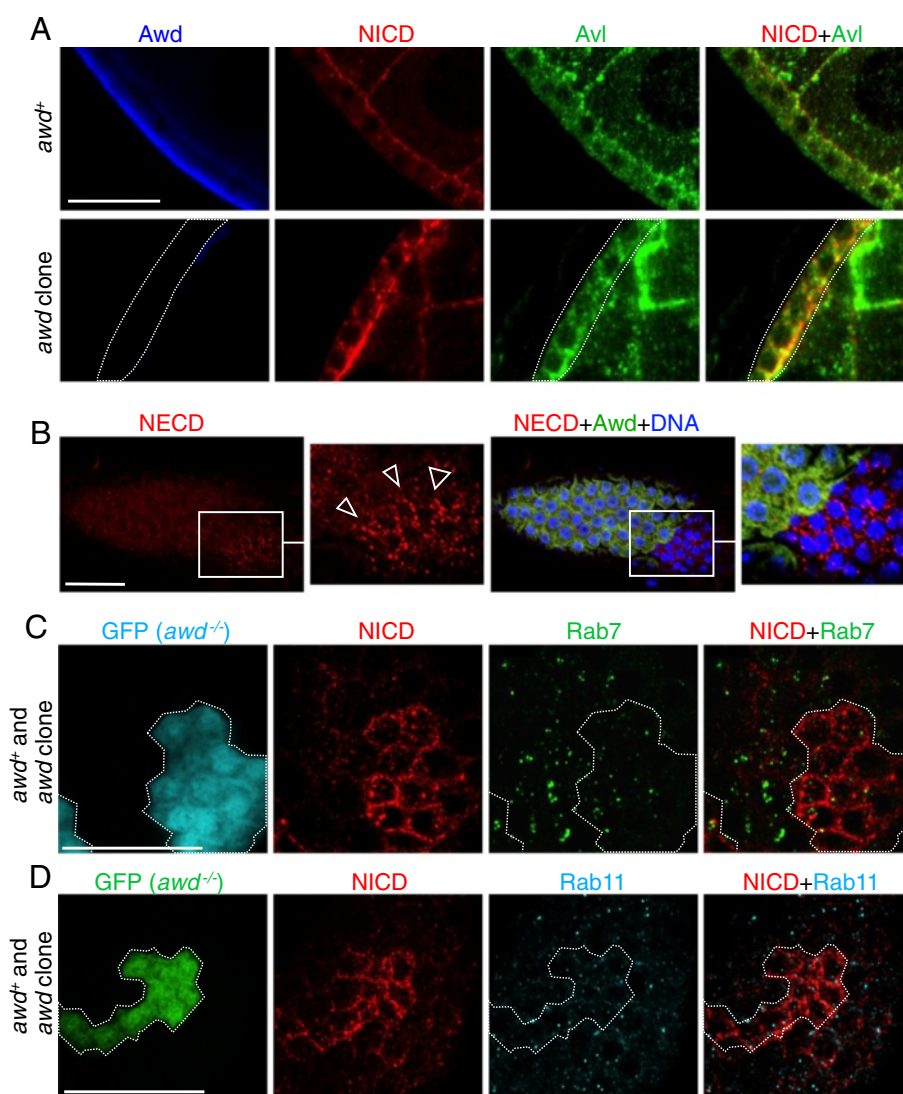
Figure 6 Notch accumulates in early endosomal compartments in awd mutant cells. (A) Stage 8 egg chambers were dissected from yw (wild-type; upper panel) or yw; en2.4-Gal4 UAS-flp/+ ; FRT 82B /FRT 82B , awd Δ2A4 ( awd clone, lower panel) females. In wild-type, Notch shows low level punctates that are partially co-localized with Avl. In the awd clone, most, if not all, large Notch-positive vesicles are also Avl-positive. Dashed line marks the awd clone. (B) Surface view of stage 7 egg chamber dissected from a yw; en2.4-Gal4 UAS-flp/+ ; FRT 82B /FRT 82B , awd Δ2A4 female and stained for Notch extracellular domain peptide (NECD), Awd and DNA. There is accumulation of NECD on the surface of awd mutant clones (empty arrowheads). (C-D) Stage 8 egg chambers were dissected from hs-flp/GbeSu(H) ms -lacZ; act-Gal4, UAS-GFP/+; FRT 82B , act-Gal80/FRT 82B , awd Δ2A4 females. awd mutant clones were identified as GFP-expressing cells. In awd clones, over-accumulated Notch does not co-localize with Rab7 (C) or Rab11 (D). Bars are 20 μm. Avl, avalanche; Awd, abnormal wing disc.
