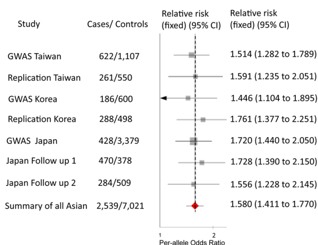
Figure 1. Per-cohort analysis of BLK rs2736340. Boxes indicate the odds ratio for each cohort, and horizontal lines denote the 95% confidence interval for the corresponding odds ratio. Diamonds represent summary odds ratios for the respective meta-analyses. Solid vertical line indicates an odds ratio of 1.0, and dashed vertical line denotes the odds ratio obtained from meta-analysis of all samples. doi:10.1371/journal.pone.0072037.g001
