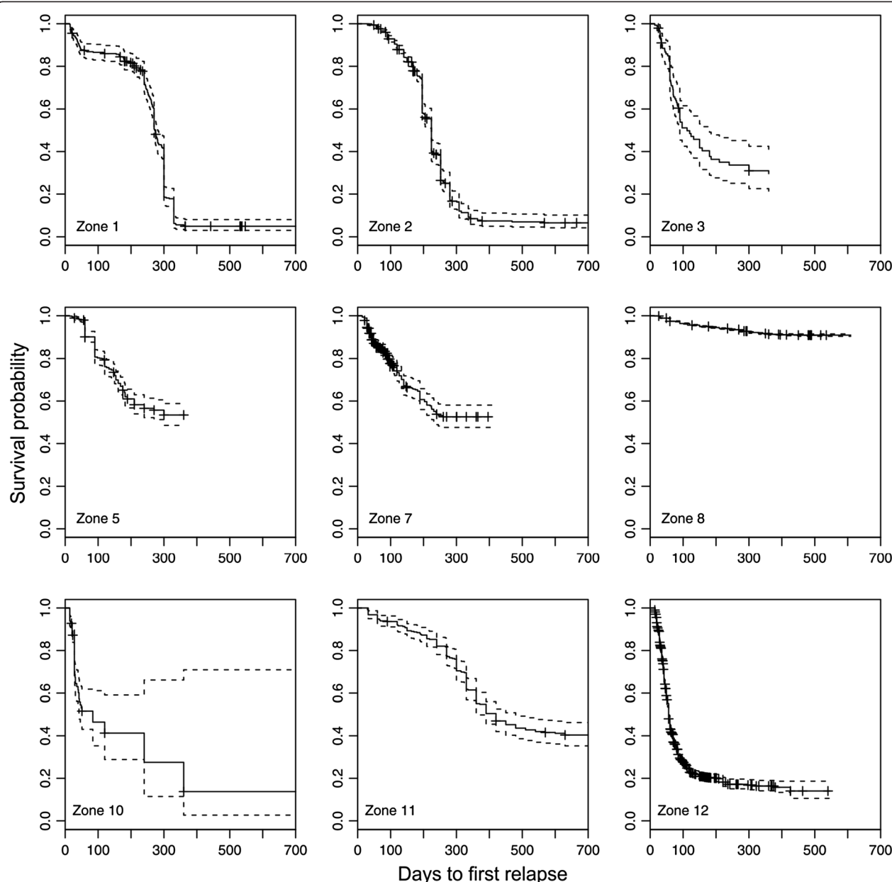
Figure 6 Survival curves for the modified Macdonald system. Shown are the Kaplan-Meier estimates (solid lines) with 95% confidence intervals (dotted lines). For each curve, all individual-level data from the respective zone have been pooled. The curves terminate at the longest follow-up day in each zone. The ticks indicate censoring events, i.e., losses to follow-up or the completion of a study without relapse. Zone 1: North America, zone 2: Central America, zone 3: South America, zone 5: Mediterranean and North Africa, zone 7: sub-Saharan Africa, zone 8: Monsoon Asia, zone 10: Southeast Asia, zone 11: northern Europe and Asia, zone 12: Melanesia.
