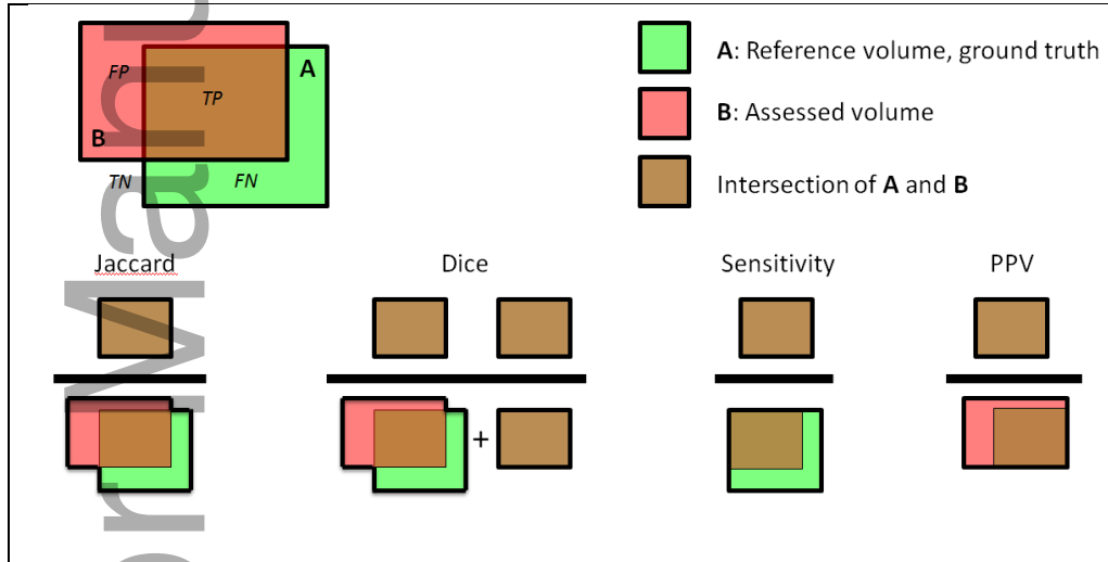
Fig. A1. A graphical illustration of the Jaccard and the Dice similarity coefficients, and of the sensitivity and the positive predictive value (PPV).
