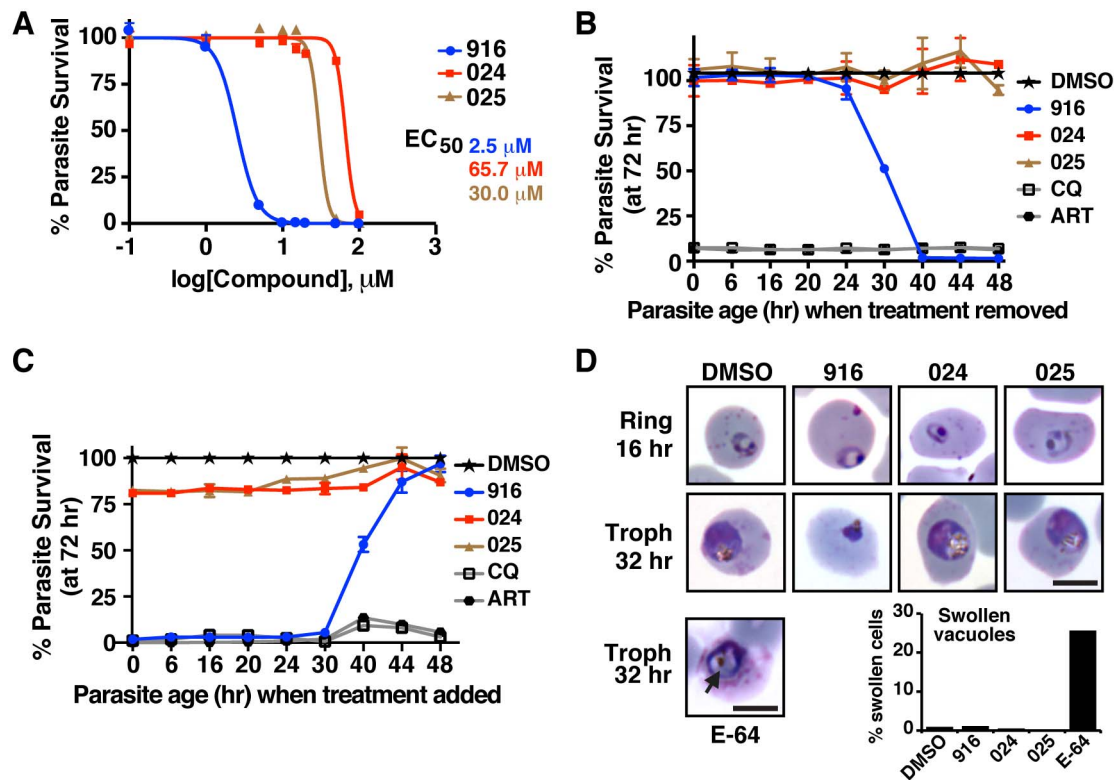
Figure 4. WEHI-916 is lethal to P. falciparum 3D7. (A) Dose-response curves of P. falciparum 3D7 in the presence of 916, 024, or 025. EC 50 values are shown. (B) Parasitemia measured at 72 h (y-axis) following drug treatment at rings (30 min postinvasion) and replacement of the medium with inhibitor-free medium (wash-out) at the time intervals shown (x-axis). (C) Parasitemia at 72 h (y-axis) after replacement of inhibitor-free medium with media containing compounds at the intervals shown (x-axis). Parasitemia was determined by FACS in (A–C) and is relative to DMSO treatment in (B) and (C). Concentrations are as follows: 916, 024, 025 (15 \mu M); CQ, chloroquine (150 ng/ml); ART, artemisinin (100 ng/ml). Error bars in (A–C) are mean \pm SEM from duplicate experiments. (D) Light micrographs of Giemsa-stained parasites 16 and 32 h after drug treatment at early rings (15 \mu M). 916-treated parasites failed to develop into trophozoites and did not recover. Ring parasites treated with E-64 (10 \mu M) [22] contained swollen food vacuoles (arrow) due to inhibition of proteases involved in hemoglobin degradation; however, treatment with DMSO, 916, 024, or 025 did not cause swelling. Swelling was quantified using 500 infected cells per condition in duplicate. Scale bar is 6 \mu m.
