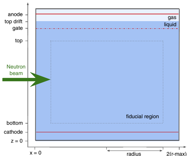
FIG. 5. Cross sectional geometry of a liquid xenon TPC (not to scale), where cylindrical symmetry is assumed. Dimensions for the detector modeled in this work are given in Table II.
