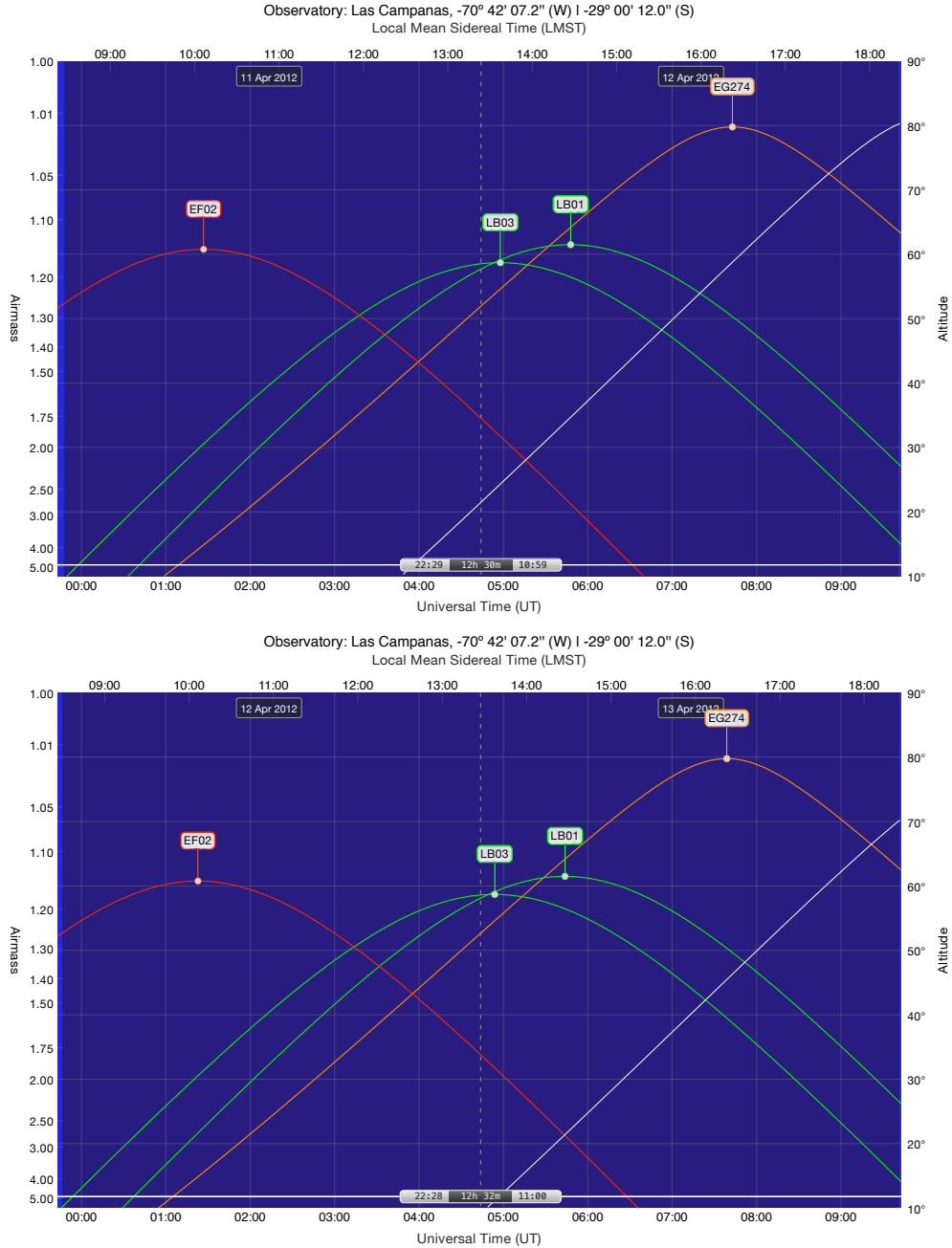
Figure 4.4: Observed object airmass tracks for April 11 th and 12 th , 2012. The red line is the airmass track of the ‘faint’ object EF02, the green lines are the airmass tracks for the ‘bright’ objects LB01 and LB03, and the orange line is the airmass track for the reference star EG 274. The white line shows the airmass track of the Moon. Image prepared using iObserve: http://www.onekilopars.ec/iobserve/ .
