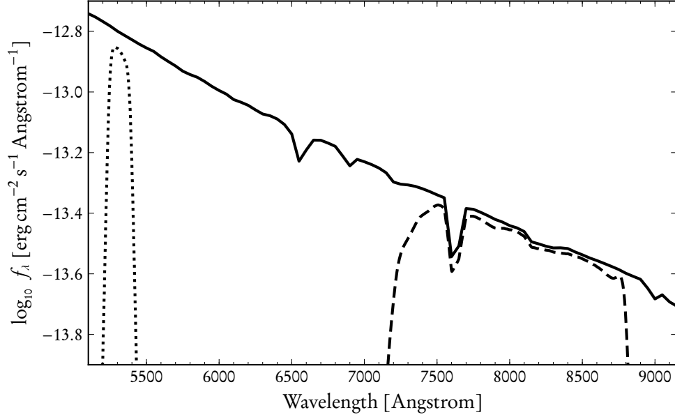
Figure 5.1: Spectral wavelength flux of reference star EG 274 as measured by Hamuy et al. (1994). For reference, the dotted line is the portion of this flux transmitted by the 5290 Å MMTF blocking filter, and the dashed line is portion transmitted by the CTIO I f/2 filter.
