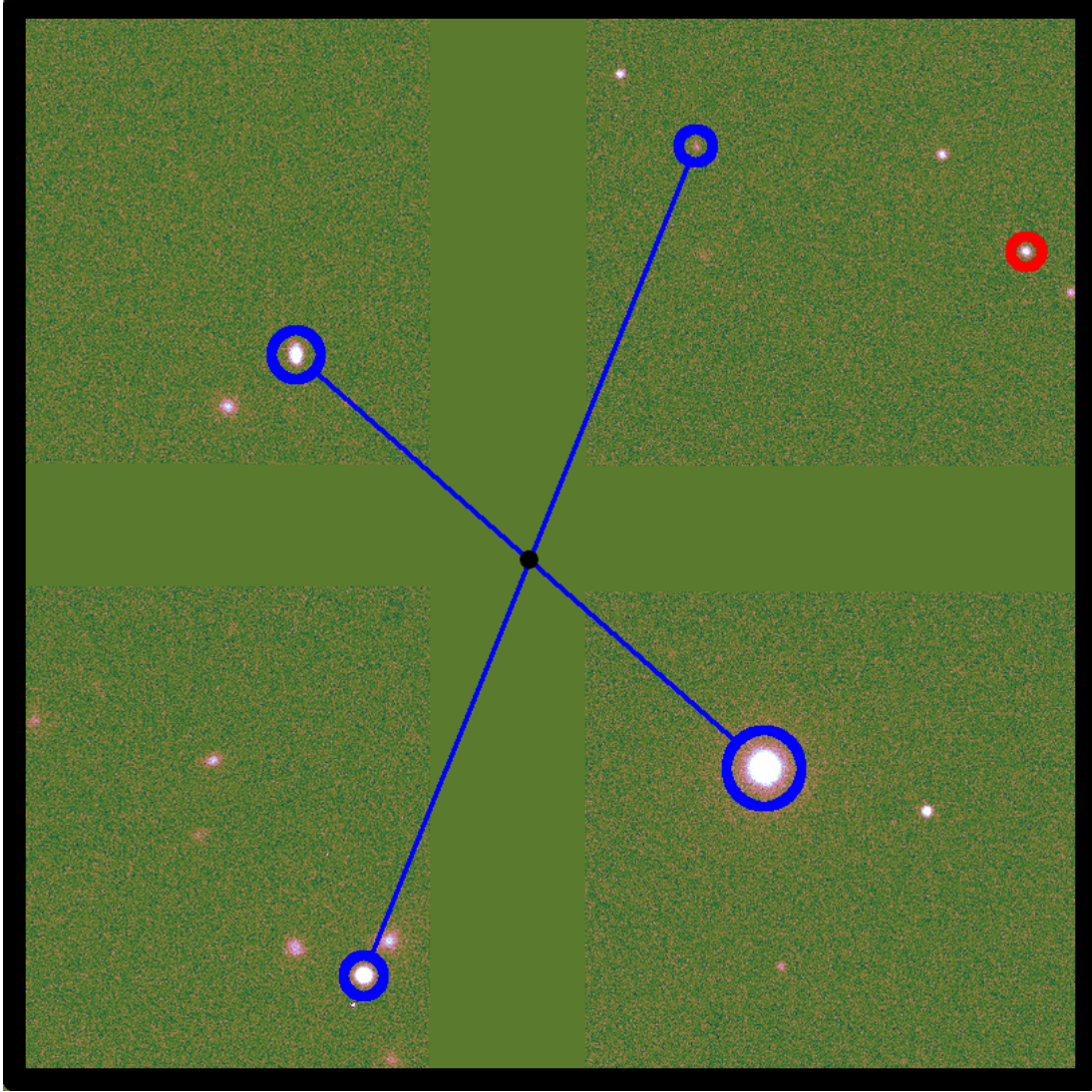
Figure 5.4: Ghost stellar images in a 5260 \text{ \AA} exposure of the EF02 field. The black dot in the centre is the optical axis, and the blue circles and lines link the saturated stellar objects (in the lower half of the image) with their ghosts. The horizontal and vertical stripes are the chip gaps on the Mosaic2 camera. The red circle in the top right is the EF02 quasar, located at (10^{\circ}6'43.8'', 0^{\circ}13'48.4'') .
