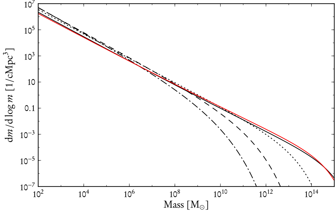
Figure 3.1: Halo mass function of the form dn/d \log m at z = 0, 2.2, 6 , and 10 (the black solid, dotted, dashed, and dash-dotted curves respectively) using the f_{\text{SMT}}(\sigma, z) mass function. For reference the solid red curve shows the halo mass function using f_{\text{PS}}(\sigma, z) at z = 0 .
