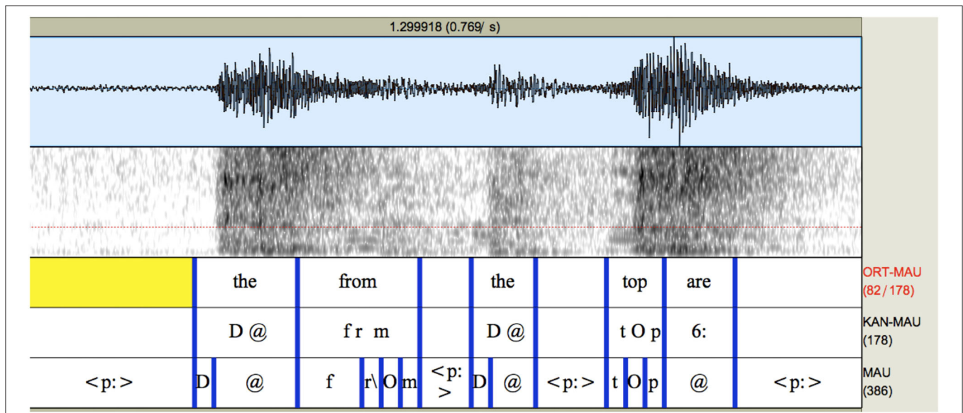
FIGURE 4 | Example 2 of system output with the poor quality recording using WEBMINNI, forced-alignment.
