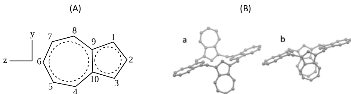
Figure 1: Structures. (A) azulene coordinate framework, and (B) calix[4]azulene in its two most stable conformations: (a) of C_i symmetry and (b) of C_s symmetry (from RSC Adv. 5 , 54848 (2015) – Published by the Royal Society of Chemistry. Ref. 9.)
