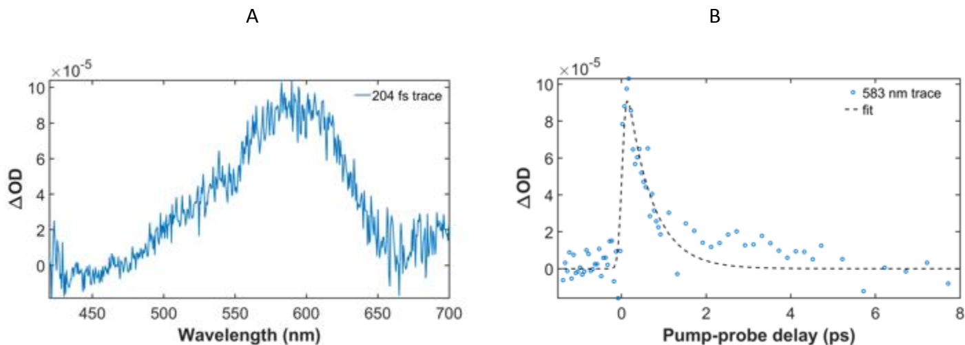
Figure 4: (A) Spectrum of the transient 204 fs following excitation of calix[4]azulene in acetonitrile (absorbance of 0.18) by 60 fs pulses at 400 nm. (B) Fit of the transient decay at 583 nm to a single exponential function; \tau = 0.6 \pm 0.3 ps (see text).
