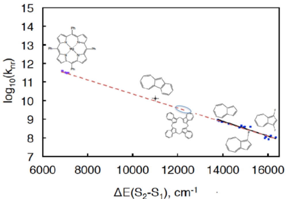
Figure 3: Energy gap law plot of the \log_{10} of the S_2 - S_1 radiationless decay constant, k_{nr} , vs. the electronic energy spacing between S_2 and S_1 for known systems in which the S_2 and S_1 states are “nested” and hence weakly coupled (Ref. 5). The expected range of data for the calixarene, if S_2 and S_1 are weakly coupled, is indicated by the oval.
