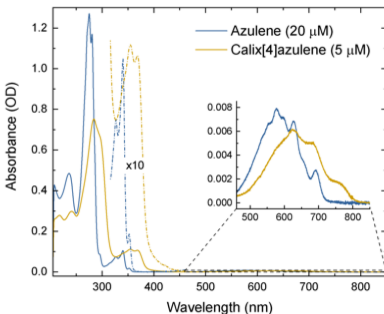
Figure 2: Absorption spectra of calix[4]azulene (5 \mu\text{M} ) in THF compared with azulene in THF (20 \mu\text{M} ) at room temperature. The backgrounds due to the absorption of the solvents in the UV have been subtracted. The short wavelength cutoff (10% transmission in a 1 cm cell) is 233 nm for pure THF. Spectra in other solvents are in the Supplementary Materials, Figure S4.
