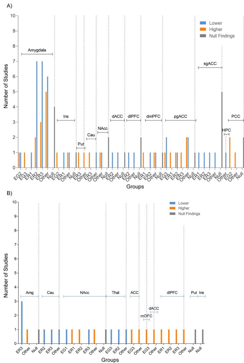
Fig. 3. Aberrant resting state functional connectivity. Histograms illustrating the number of studies that showed depression (A) and substance use (B) associated aberrant resting state functional connectivity between seed regions and EG1 (amygdala), EG2 (insula), EG3 (basal ganglia), ER1 (dmPFC/dACC/SMA/Pre-SMA), ER2 (dlPFC/vlPFC/IOFC), ER3 (rACC/vmPFC/mOFC/hippocampus) and other regions. Orange bars represent higher connectivity and blue bars represent lower connectivity. Gray bars represent null findings for each seed region. (For interpretation of the references to colour in the Figure, the reader is referred to the web version of this article).
