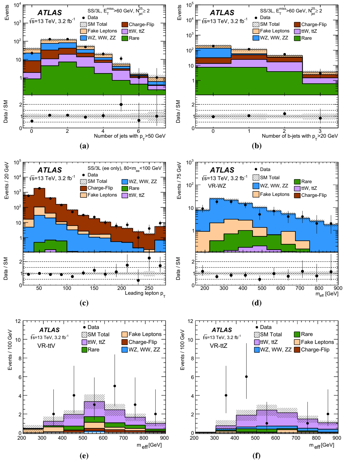
Fig. 2 Distributions of kinematic variables after a SS/3L selection including a, b E_T^{\text{miss}} > 60 \text{ GeV} and N_{\text{jet}}^{25} \geq 2 , c a b -jet veto and 80 < m_{\ell\ell} < 100 \text{ GeV} , and d-f distributions in the validation regions. The statistical uncertainties in the background prediction are included in the uncertainty band, as well as the theory uncertainties for the backgrounds with prompt SS/3L, and the full systematic uncertainties for
