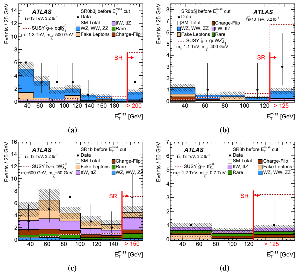
Fig. 3 Missing transverse momentum distributions after a SR0b3j, b SR0b5j, c SR1b and d SR3b selection, beside the E_T^{\text{miss}} requirement. The results in the signal regions are shown in the last (inclusive) bin of each plot. The statistical uncertainties in the background prediction are included in the uncertainty band, as well as the theory uncertainties
