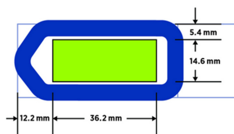
Figure 2. Slide dimensions and tissue placement for GeoMx DSP study. Tissue sections must be placed in the digital scan area (shown in green), measuring, at maximum, 36.2 mm long by 14.6 mm wide in the center of the slide. The tissue sections should not overlap the slide gasket (shown in blue) or the tip calibration area (the triangular region to the left of the green scan area). The frosted/label end of the slide is on the right.
