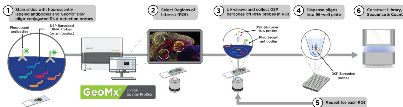
Figure 1. GeoMx workflow with NGS readout. The sequence of steps in the GeoMx workflow may be grouped into three phases: slide preparation (1), GeoMx instrument run (2–5) and readout (6). During slide preparation, a high-plex mixture of photocleavable oligo-linked probes (RNA shown) and morphology reagents are applied to the tissue section (1). Slides are loaded into the GeoMx instrument for a series of automated steps. After the researcher selects ROIs (2), the GeoMx instrument illuminates each area-of-illumination (AOI) with UV light to collect and deposit the photo-released oligos into a microtiter plate (3,4). Collection is repeated (5) to produce an AOI collection plate, where each well corresponds to a pool of photocleaved oligos from one AOI on the tissue. For NGS readout (6), each AOI (or well) is uniquely indexed during library preparation and can be pooled into one sequencing run.
