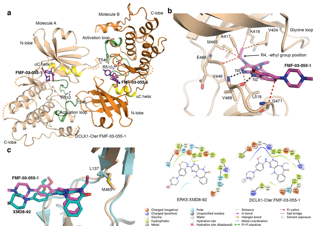
Fig. 3 Structure of DCLK1-Cter:FMF-03-055-1. a The structure of two molecules of DCLK1-Cter:FMF-03-055-1 within the asymmetric unit in a “head-to-tail” arrangement. b Close up of the interaction of DCLK1-Cter with FMF-03-055-1. c Overlay of DCLK1-Cter:FMF-03-055-1 with ERK5:XMD8-92 showing the differences in the gatekeeper residues, Leu137 in ERK5 and Met 465 in DCLK1 and ligand interaction diagrams generated using Schrödinger Maestro, including prediction of protonation states at pH 7.0 using Epik (Release 2020-3; Schrödinger, LLC, New York, NY, 2020). The h-bond and vdw interaction are shown in black and red dashed lines, respectively. The flexible residues in DCLK1-Cter: FMF-03-055-1 are shown in orange dashed lines. FMF-03-055-1, magenta; XMD8-92, teal.
