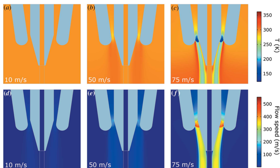
Figure 8 (a)–(c) Simulated temperature and (d)–(f) velocity profiles of a nitrogen sheath gas surrounding a capillary with a 75 \mu\text{m} internal diameter. Gas flow speed is 10 \text{ m s}^{-1} in (a) and (d); 50 \text{ m s}^{-1} in (b) and (e); and 75 \text{ m s}^{-1} for (c) and (f).
