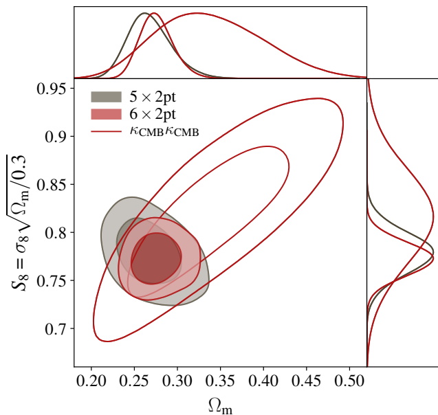
FIG. 4. Marginalized constraints on \Omega_m and S_8 \equiv \sigma_8 \sqrt{\Omega_m/0.3} for different combinations of correlation functions in the context of \Lambda CDM+ \nu cosmology: 5 \times 2 pt (gray), \kappa_{\text{CMB}}^{\kappa_{\text{CMB}}} (open red) and 6 \times 2 pt (red). The w^{\kappa_{\text{CMB}}^{\kappa_{\text{CMB}}}} contours are derived from the Planck 2015 lensing data [21]. The 5 \times 2 pt contours are identical to those in Fig. 2. The \kappa_{\text{CMB}}^{\kappa_{\text{CMB}}} constraints are complementary to those of the 5 \times 2 pt analysis.
