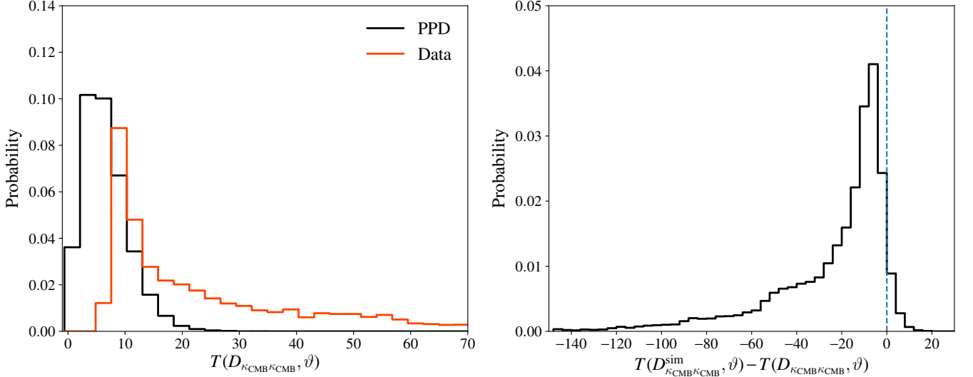
FIG. 6. Same as Fig. 5, except now showing results of PPD analysis to assess consistency between 5\times 2 pt data vector and w^{\kappa_{\text{CMB}}\kappa_{\text{CMB}}}(\theta) data vector. In this case, approximately 9% of the simulated realizations of w^{\kappa_{\text{CMB}}\kappa_{\text{CMB}}}(\theta) lead to a test quantity that is greater than that of the actual data. This indicates that w^{\kappa_{\text{CMB}}\kappa_{\text{CMB}}}(\theta) is statistically consistent with the 5\times 2 pt data vector under the flat \Lambda\text{CDM} model.
