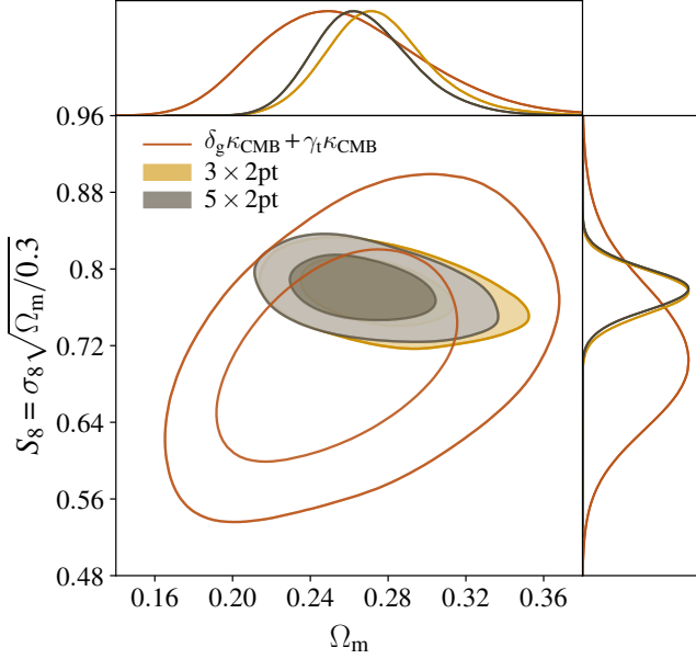
FIG. 2. Marginalized constraints on \Omega_m and S_8 \equiv \sigma_8 \sqrt{\Omega_m/0.3} for different combinations of correlation functions in the context of \Lambda\text{CDM}+\nu cosmology: 3\times 2\text{pt} (gold), w^{\delta_g^{\kappa\text{CMB}}}(\theta) + w^{\gamma^{\kappa\text{CMB}}}(\theta) (open orange) and 5\times 2\text{pt} (gray). We note that the w^{\gamma^{\kappa\text{CMB}}}(\theta) + w^{\delta_g^{\kappa\text{CMB}}}(\theta) constraints have a different degeneracy direction compared to those of 3\times 2\text{pt} .
