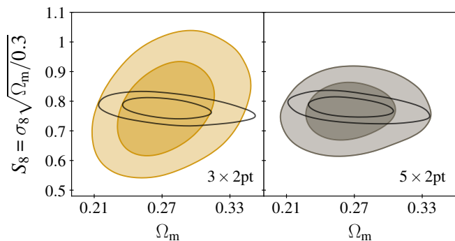
FIG. 3. Marginalized constraints on \Omega_m and S_8 \equiv \sigma_8 \sqrt{\Omega_m/0.3} for the 3 \times 2pt (gold) and 5 \times 2pt (gray) combinations of correlation functions in the context of \Lambda CDM+ \nu cosmology when priors on multiplicative shear bias are relaxed (filled contours). In this case, the cosmological constraints obtained from the 5 \times 2pt data vector are significantly tighter than those resulting from the 3 \times 2pt data vector. The open black contours show the constraints when the fiducial priors on multiplicative shear bias (see Table I) are applied.
