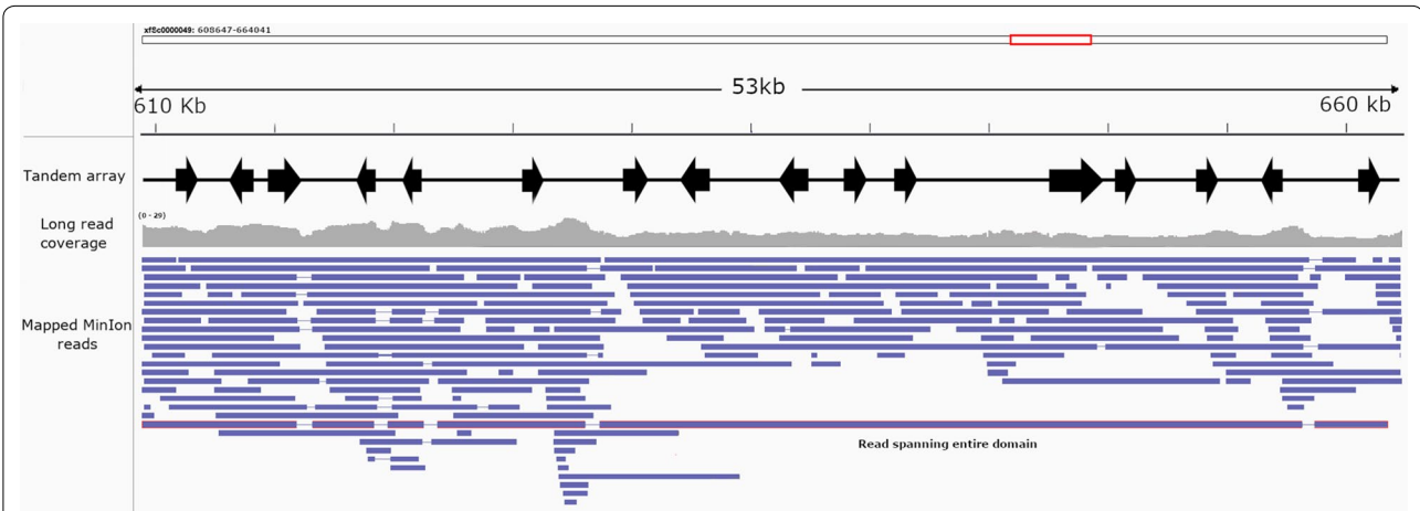
Fig. 2 Representation of the SCP/TAPS tandem array in L. cuprina . A 53 kb region of scaffold xfs0000049 containing a tandem array of 16 SCP/TAPS genes. Genes (black arrows with transcription orientation indicated by arrow), Oxford Nanopore MinION mapped long reads (blue) with associated coverage plot (grey) are pictured. A mapped long read is shown depicted with a red outline highlighting that a single read spans the entire tandem array
