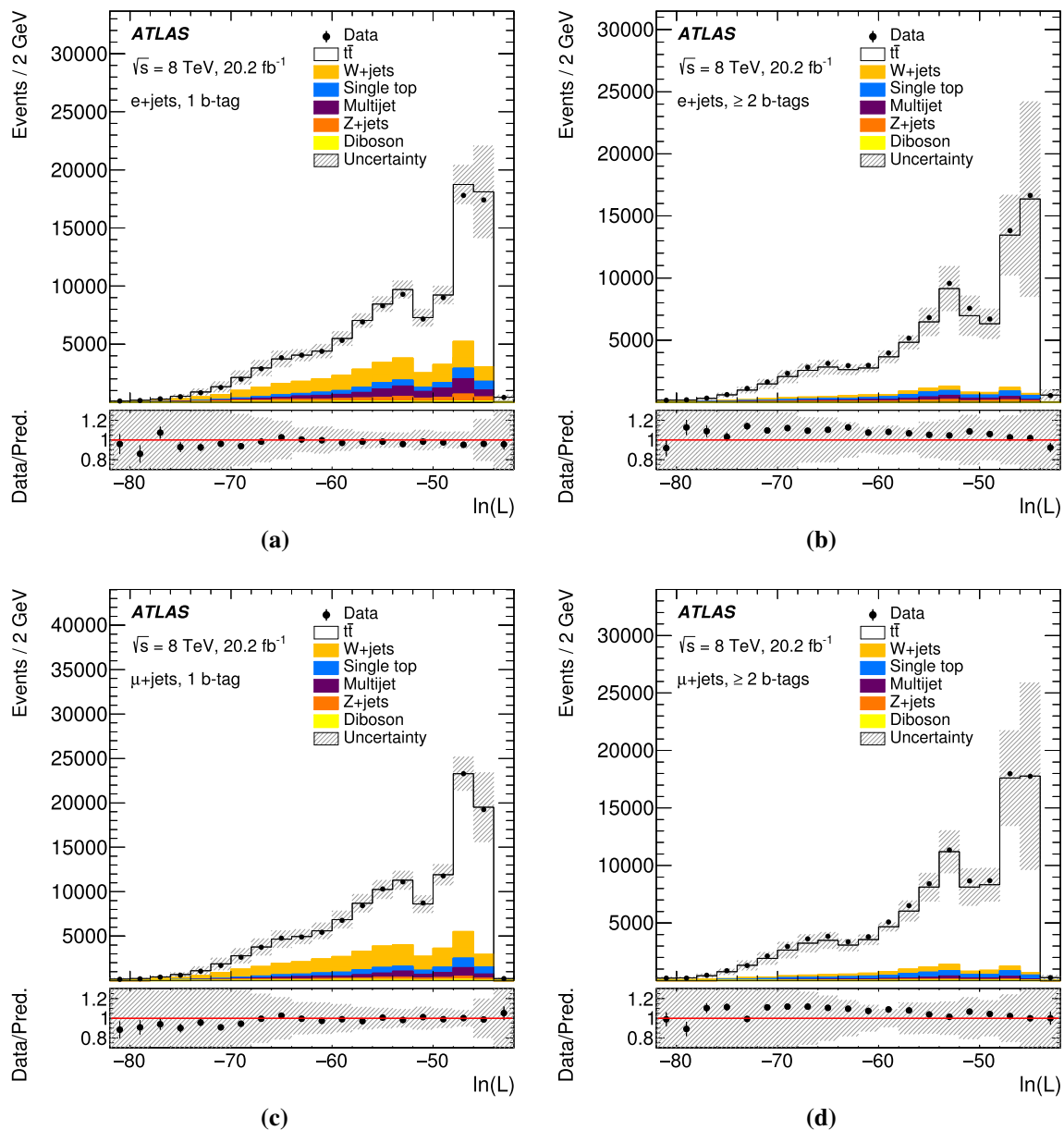
Fig. 3 Distributions of the logarithm of the likelihood obtained from the event reconstruction algorithm for the selected a , b electron+jets and c , d muon+jets events with a , c exactly one and b , d at least two b -tagged jets. The hatched bands show the normalisation uncertainty in
