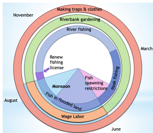
APV_12256_Figure_2_Fishing_livelihoods_calendar_Radford_&_Lamb300.tiff
