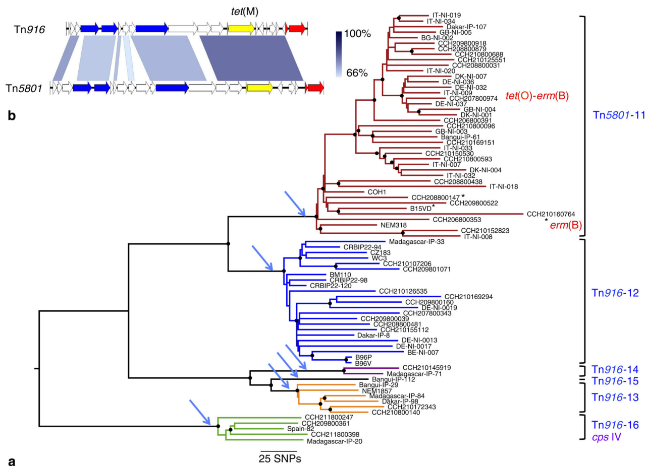
Figure 3. Phylogeny of the 'hypervirulent' CC17 lineage
