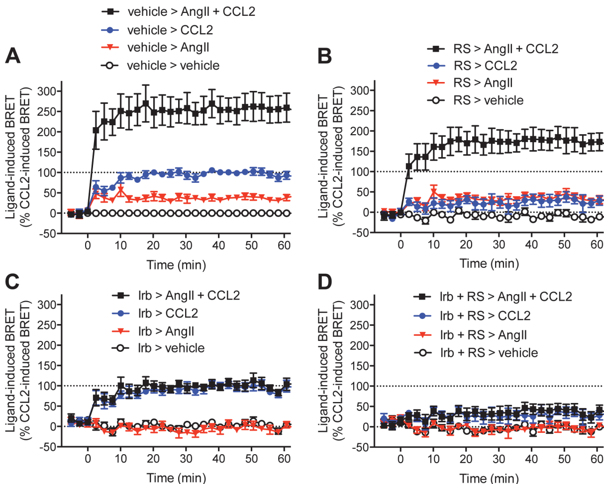
Fig 4. Effect of combined AT 1 receptor and CCR2 blockade on GPCR-HIT with \beta -arrestin2. Real-time kinetic profiles were generated with live HEK293FT cells co-expressing CCR2-RLuc8, \beta -arrestin2-Venus and AT 1 receptor with 30 min preincubation at 37°C with vehicle (A), RS504393 (RS; 10 \mu M; B), Irbesartan (Irb; 10 \mu M; C), or both combined (D). Cells were then stimulated with AngII and/or CCL2 (100 nM) and BRET signals measured. 100% is defined as the mean increase in BRET signal observed 20 min after addition of CCL2 and following preincubation with vehicle. Data are presented as mean \pm SEM of five independent experiments.
