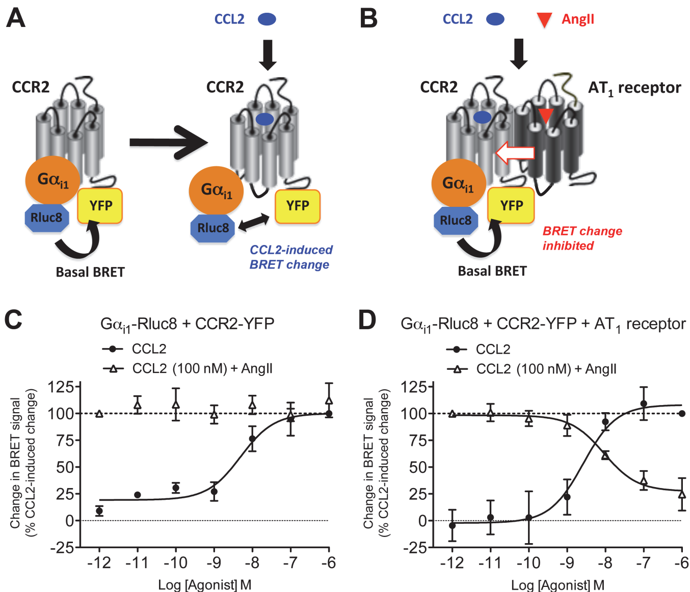
Fig 1. Use of GPCR-HIT to show effect of AT 1 receptor activation on CCR2/G \alpha_{i1} proximity. Live HEK293FT cells co-expressing G \alpha_{i1} -Rluc8 with either CCR2-YFP only (A and C) or CCR2-YFP and AT 1 receptor (B and D) were used to measure the change in BRET signal with increasing doses of CCL2, or 100 nM CCL2 with increasing doses of AngII (C and D). It has been observed previously [39,41,42,44] that the BRET signal can increase or decrease as a consequence of the ligand-induced conformational change associated with G \alpha_{i1} protein activation (A). The data are presented here as change in BRET signal as a percentage of CCL2-induced change for ease of interpretation. 100% is defined in each individual experiment as the decrease in BRET signal observed upon addition of 1 \mu M CCL2 (for curves with black circles), or 100 nM CCL2 + 1 pM AngII (for curves with white triangles). Data are presented as mean \pm SEM of three (C) or five (D) independent experiments. CCL2 logEC 50 in (C) = -8.27 \pm 0.20 and in (D) = -8.67 \pm 0.13 (not significantly different (unpaired t-test, P > 0.05 )). In the presence of AT 1 receptor, logIC 50 for AngII inhibiting 100 nM CCL2 = -8.19 \pm 0.31 .
