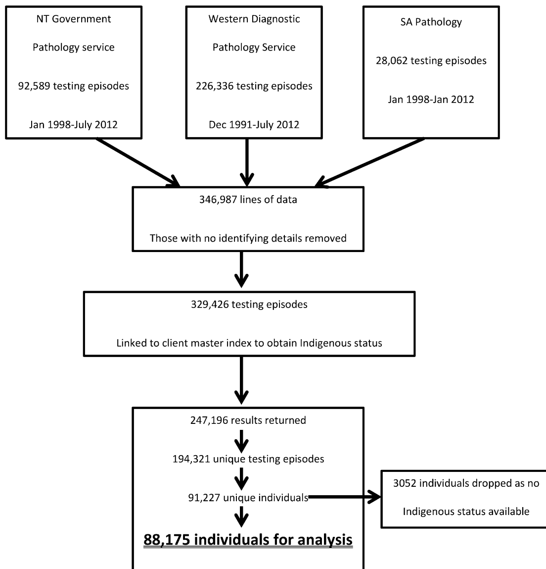
Fig 1. Flow diagram detailing sources of testing data and production of dataset including only the latest set of results for each individual with all the duplicate tests and individuals removed.
