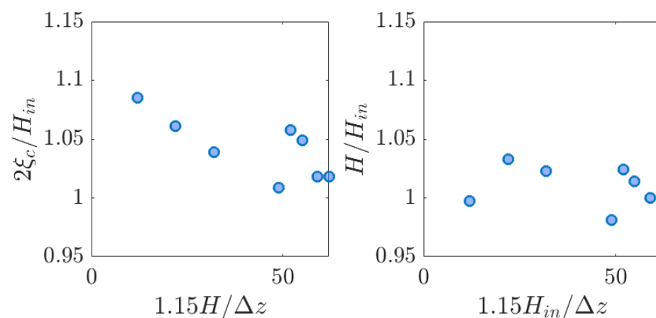
Figure A1. Mesh study performed to find the grid that can be used for simulating the problem. Left and right panels respectively show the recorded wave crest height and wave height. The results presented in this figure correspond to water waves with a period of 0.8 s and a wave height of 0.035 m.
