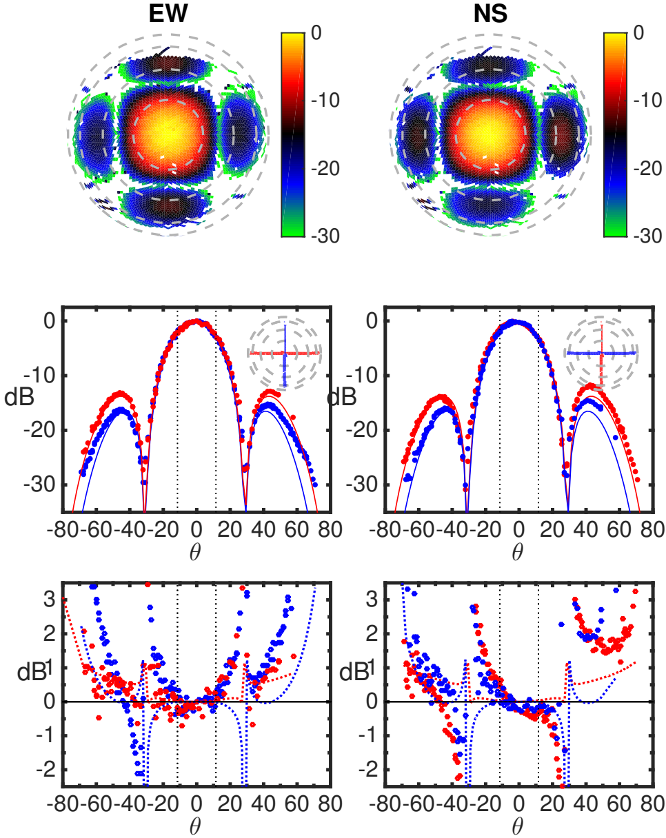
Figure 6. The measured MWA tile beampattern for the zenith pointing is plotted in dB relative to its bore-sight gain (top). Beams of the EW (NS) oriented antennas are shown in the left (right) column. The maps are in sine projection with North at the top and East at the right. Dashed circles mark 20, 40, 60, and 80 degrees from zenith. We show measured and model beampatterns (middle) and deviations from the model (bottom) on slices through the E (red) and H (blue) antenna planes. Dashed lines in the bottom panel show the model of Sutinjo et al. [2015] relative to the analytic model. Vertical dotted lines mark the model FWHM of \sim 23 degrees at 137 MHz.
