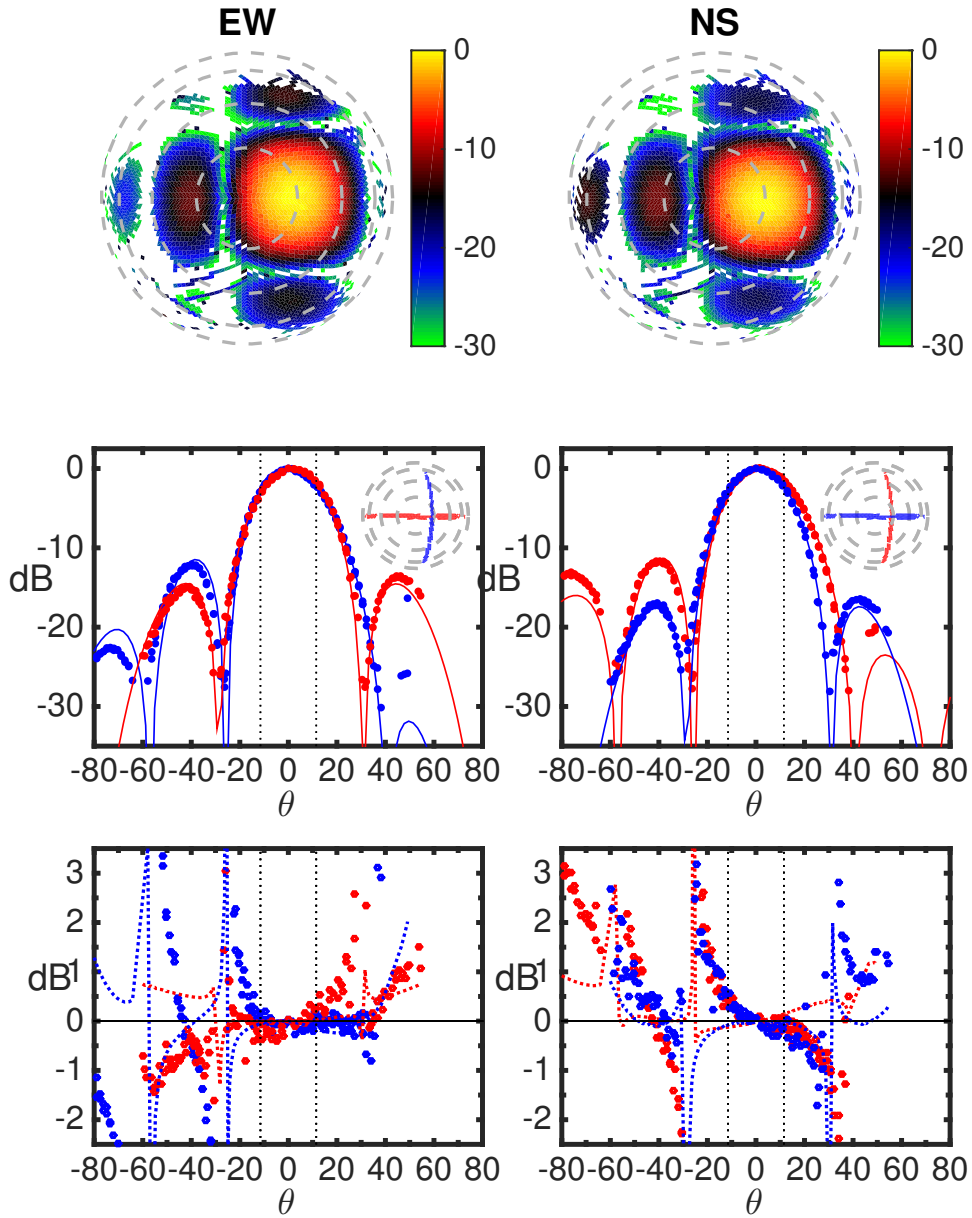
Figure 8. Measured MWA tile power pattern for pointed 20 degrees East pointing. Same layout as Figure 7.
