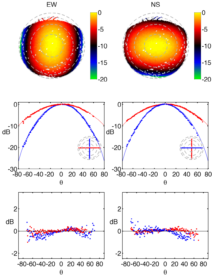
Figure 4. Results from our null experiment in which the AUT is another reference antenna. Beams of the EW (NS) oriented dipoles are shown in the left (right) column. The measured AUT beampattern is plotted in dB relative to its boresight gain (top). These maps are in sine projection with North at the top and East at the right. Dashed circles mark 20, 40, 60, and 80 degrees from zenith. We also show measured and model beampatterns (middle) and deviations from the model (bottom) on slices through the E (red) and H (blue) antenna planes.
