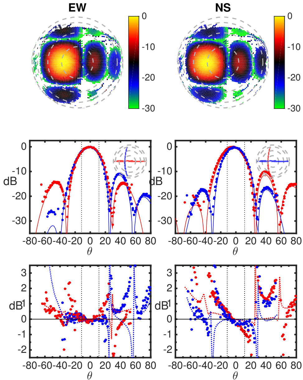
Figure 7. Measured MWA tile power pattern for pointed 20 degrees West pointing. Same layout as Figure 6, except here we plot beam slices through orthogonal planes through the main lobe (red and blue) which do not correspond to the E and H antenna planes because the direction of boresight is no longer in these planes.
