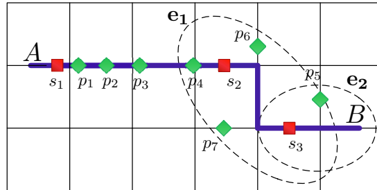
Fig. 5. Effect of POI density on Flip-flop's search space.
