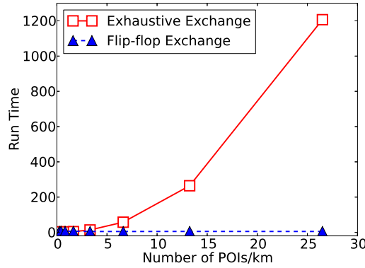
Fig. 6. Effect of POI density on Flip-flop's performance.
