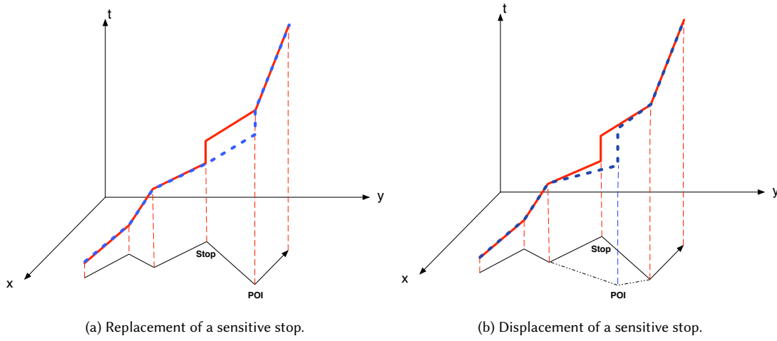
Fig. 3. Strategies to protect sensitive stops.
