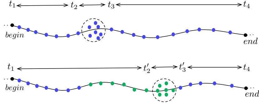
Fig. 1. Protecting stops through exchanging trajectory episodes.
