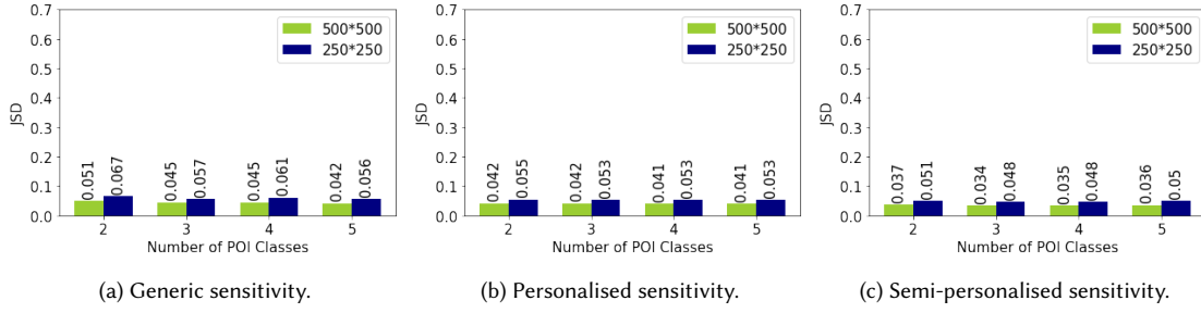
Fig. 9. Error in spatial density distribution estimation, \mathcal{E}_{density} .
