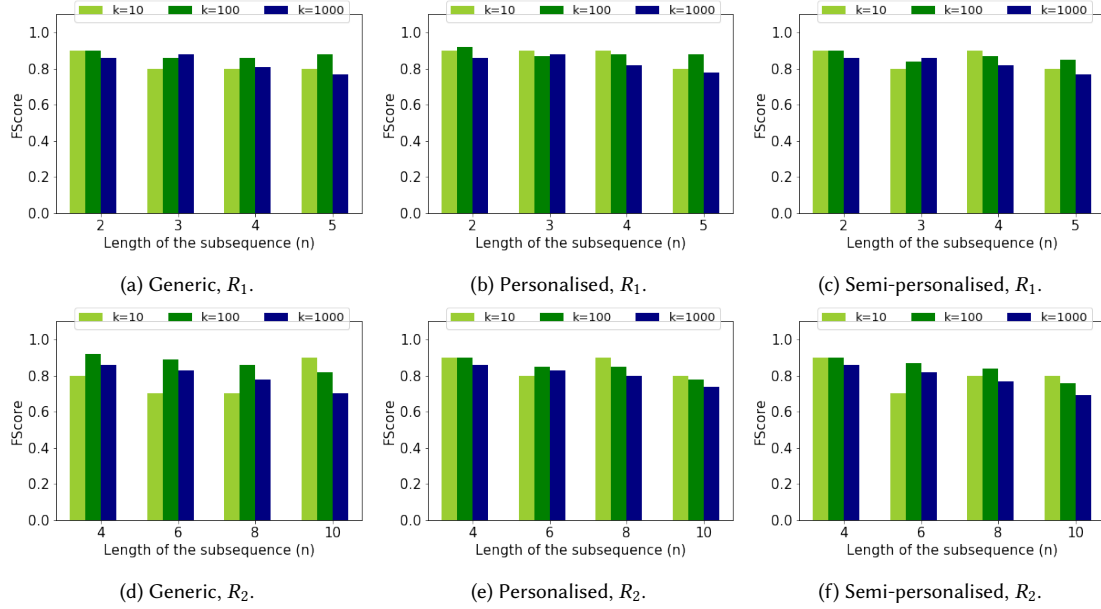
Fig. 11. Utility (similarity) of frequent spatial patterns, U_{SP} , for varying k and n when T_p = 5 .
