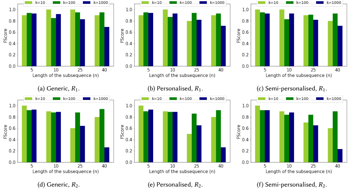
Fig. 10. Utility (similarity) of frequent spatio-temporal patterns, U_{STP} , for varying k and n when T_p = 5 .
