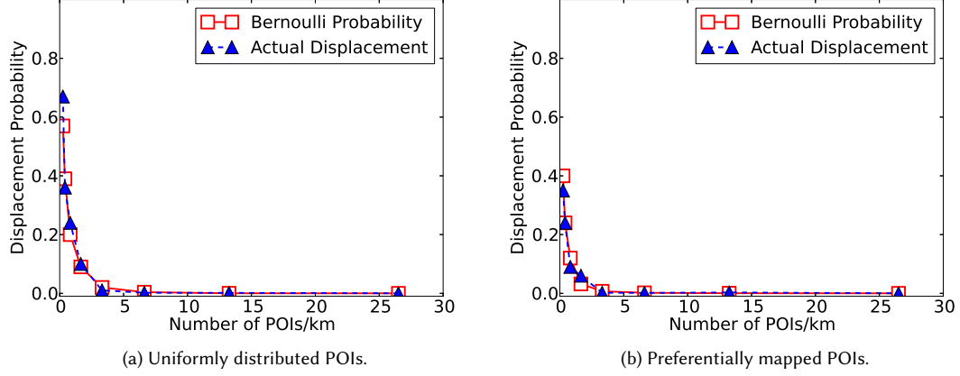
Fig. 7. Effect of POI density on displacement probability on two settings.
