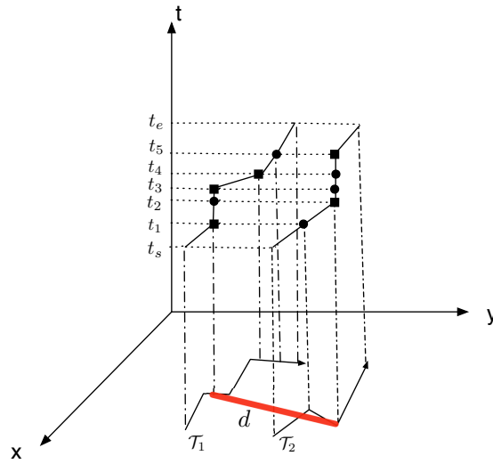
Fig. 2. Estimating the distance between trajectories after matching their timestamps.
