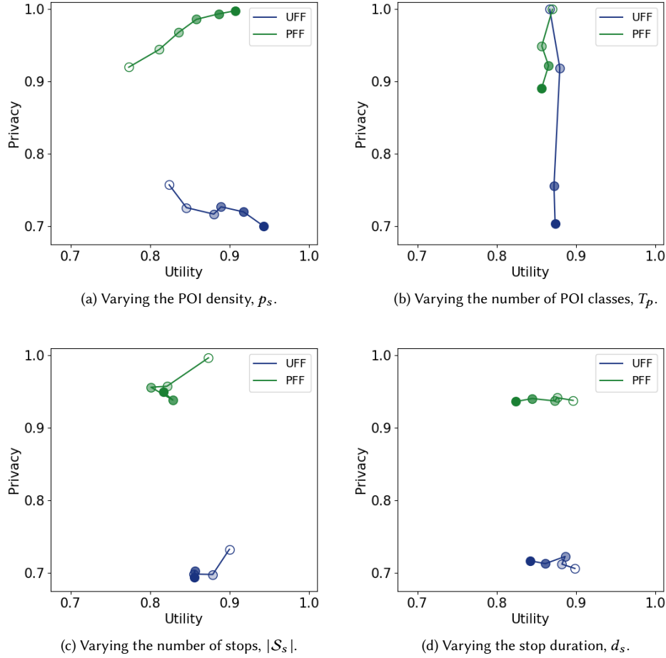
Fig. 8. The effect of varying the parameters in Table 2 on the privacy/utility balance. The change in the colors from light to dark correspond to an increase in each parameter.
