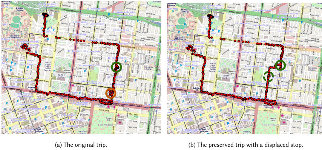
Fig. 4. A real-world trip in the city of Melbourne and its private match. Green corresponds to non-sensitive stops and orange circle corresponds to the sensitive stops. The solid circles correspond to the actual stops while the dashed circle shows the exchanged non-sensitive stop.
