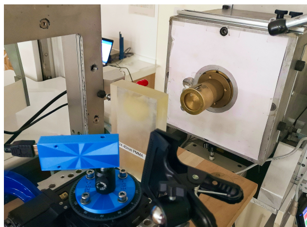
Figure 2: Experimental setup with detector angled at 45° to the beam, approximately 18 cm from the collimator. Upstream, a block of PMMA decreases the depth of the BP.
