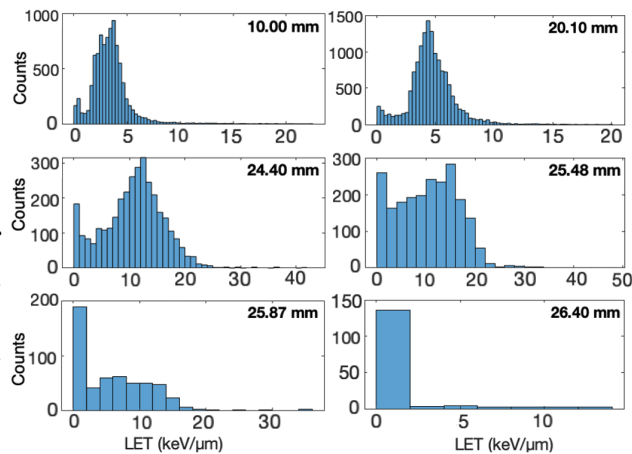
Figure 4: LET spectra with the sensor at 45°.
