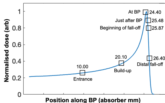
Figure 3: Observed depths along the BP for the different PMMA blocks.
