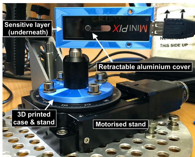
Figure 1: The MiniPIX-Timepix detector, a retractable aluminium sheath covers the chip sensitive area with the centre positioned at the the origin of the rotational axis.
