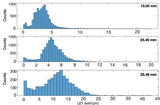
Figure 5: LET spectra with the sensor at 60°.
