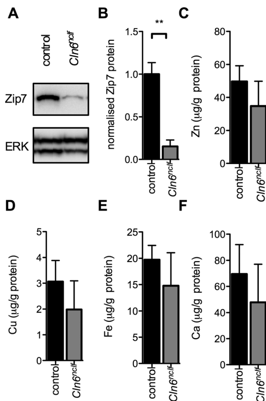
Fig. 1 Zip7 loss in CbCln6 ncif cells is not associated with altered global biometal levels. (A) Representative immunoblot of Zip7 and total ERK expression in cellular homogenates (5 μg) harvested from non-treated control and CbCln6 ncif mutant cells. (B) Densitometry analysis of immunoblots ( n = 3 biological replicates), normalized to expression of total ERK protein was performed using ImageJ. Values are mean + SEM. ** p < 0.01 by Student's t -test. (C–F) Total cellular zinc (C), copper (D), iron (E) and calcium (F) concentrations were analysed using ICP-MS. Metal concentrations are normalized to total cellular protein content, as measured by BCA assay, and are expressed as mean + SEM.
