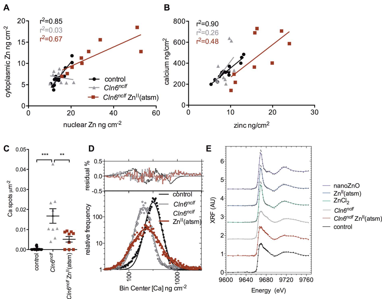
Fig. 5 Zn^{II}(\text{atSm}) treatment restores subcellular biometal homeostasis in CbCln6 nclf cells. (A) The nuclear concentration of zinc in each individual cerebellar control cell (black circles), CbCln6 nclf cell (grey triangles) and CbCln6 nclf cell treated for 2 h with 1 \mu\text{M } Zn^{II}(\text{atSm}) (red squares) was plotted against the cytoplasmic concentration of zinc in the same cell. Linear regression analysis was performed in GraphPad Prism. r^2 values for the strength of each correlation are presented. (B) The concentration of zinc in each individual control cell (black circles), CbCln6 nclf cell (grey triangles) and CbCln6 nclf cell treated for 2 h with 1 \mu\text{M } Zn^{II}(\text{atSm}) (red squares) was plotted against the concentration of calcium in the same cell. (C) Binary masks were generated to examine the number of regions of high calcium intensity (above 2 \mu\text{g cm}^{-2} ) per cell area for each treatment group. **p < 0.01 , ***p < 0.0001 by one-way ANOVA and Bonferroni multiple comparison posttests. Error bars represent SEM. (D) The histograms (tabulated frequency, bin width = 0.0385 \text{ ng cm}^{-2} ) of the log-transformed calcium concentrations in cells were modeled by Gaussian curves (solid black, grey or red lines). The residual plots are presented above the histograms. (E) Zinc K-edge XANES of control cells, CbCln6 nclf cells and CbCln6 nclf cells treated for 2 h with 1 \mu\text{M } Zn^{II}(\text{atSm}) was performed using X-rays at 59 energies ranging from 9.604 to 9.764 keV. Pre-edge absorbance values were linearized and normalized XANES is expressed as a percentage of the absorbance maxima. XANES spectra for ZnCl_2 and ZnO nanoparticles are presented as controls.
