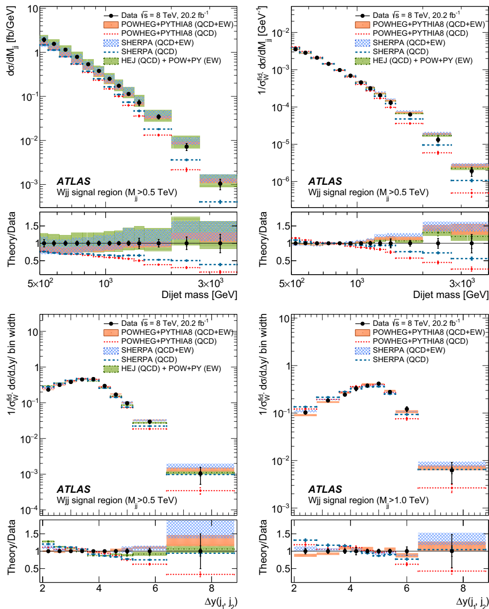
Fig. 16 Top Unfolded absolute (left) and normalized (right) differential Wjj production cross sections as a function of dijet mass for the signal fiducial region. Bottom Unfolded normalized production cross sections as a function of \Delta y(j_1, j_2) for the signal regions with
