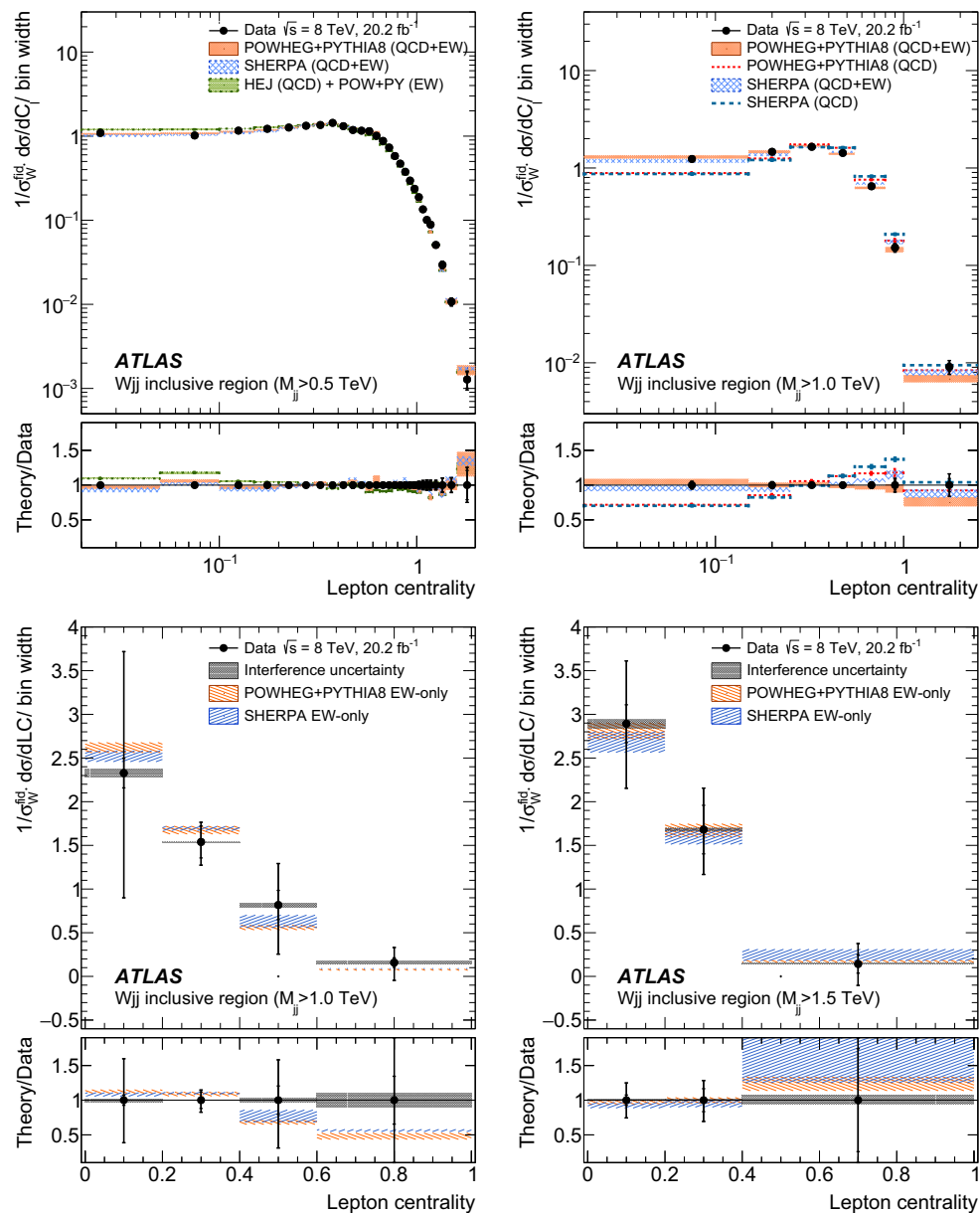
Fig. 23 Unfolded normalized differential QCD+EW Wjj (top) and EW (bottom) production cross sections as a function of lepton centrality for the inclusive fiducial region with M_{jj} > 0.5 TeV (top left), 1.0 TeV (top right and bottom left), and 1.5 TeV (bottom right). Both
