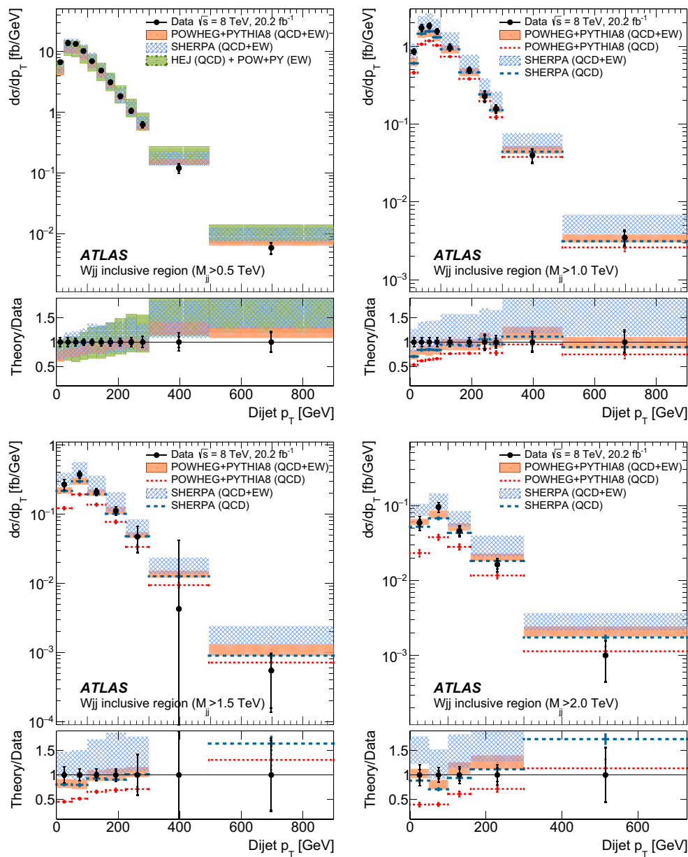
Fig. 46 Differential Wjj production cross sections as a function of dijet p_T in the inclusive fiducial region with four thresholds on the dijet invariant mass (0.5, 1.0, 1.5, and 2.0 TeV). Both statistical ( inner bar )
