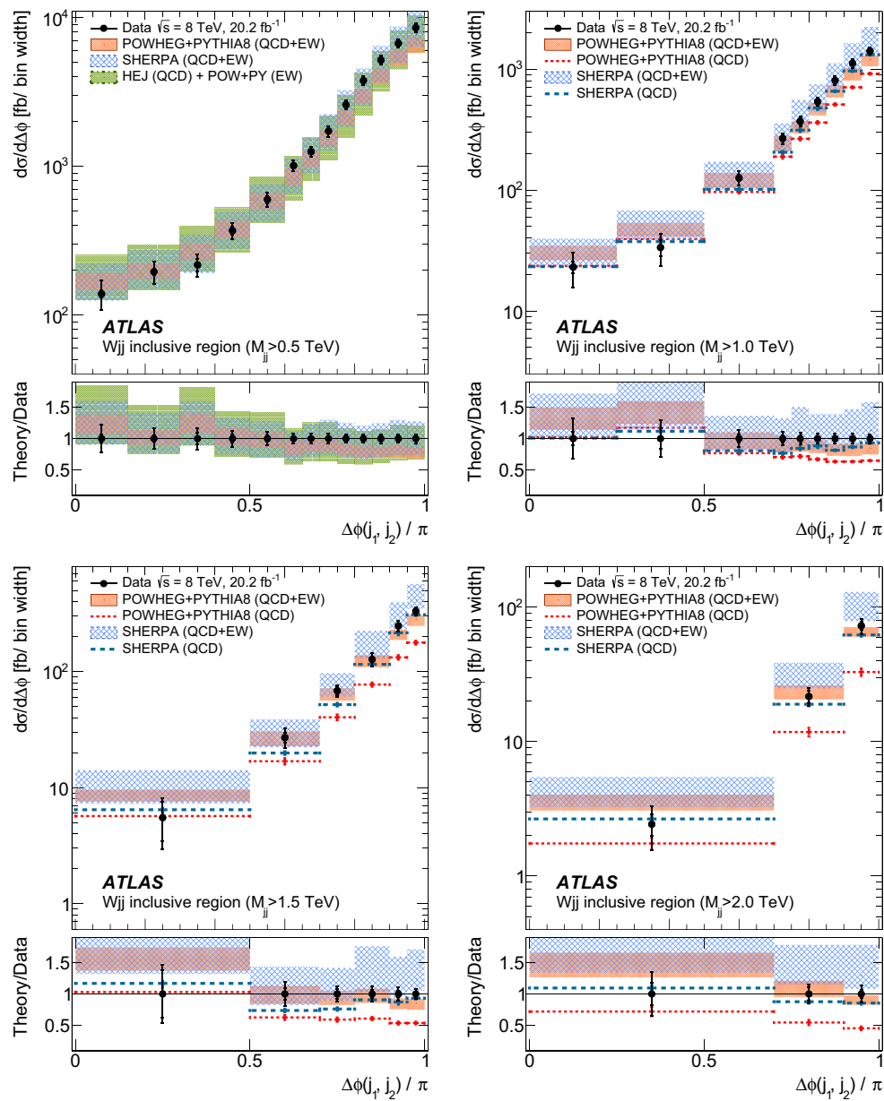
Fig. 51 Differential Wjj production cross sections as a function of \Delta\phi(j_1, j_2) in the inclusive fiducial region with four thresholds on the dijet invariant mass (0.5, 1.0, 1.5, and 2.0 TeV). Both statistical ( inner
