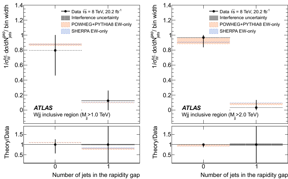
Fig. 21 Unfolded normalized differential EW Wjj production cross sections as a function of the number of jets with p_T > 30 GeV in the rapidity interval bounded by the two highest- p_T jets in the inclusive fiducial region, with M_{jj} > 1.0 TeV (left) and M_{jj} > 2.0 TeV (right).
