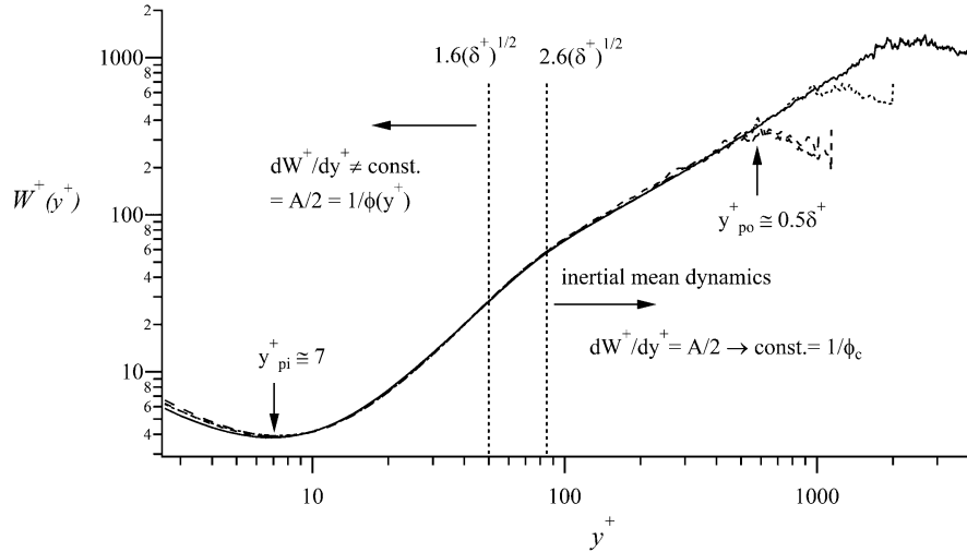
FIG. 2. Distribution of W^+(y^+) for pipe and channel flows; pipe flow DNS 41 at \delta^+ = 1142 , - · - ·; channel flow DNS 42 at \delta^+ = 1020 , - - -; channel flow DNS 43 at \delta^+ = 2004 , ·····; channel flow DNS 11 at \delta^+ = 4080 , ———. Vertical lines denoting the beginning and end of layer III are computed for \delta^+ = 1000 (see figure 1). The upper and lower bounds of the layer hierarchy correspond to the inner ( y_{pi}^+ ) and outer ( y_{po}^+ ) peaks of the TI term, or equivalently the minimum and maximum values of W^+(y^+) .
