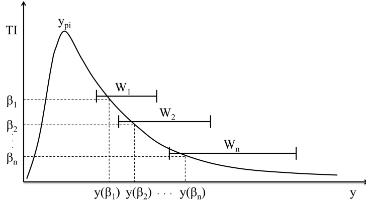
FIG. 3. Schematic depiction of the layer hierarchy described by the continuous distribution of widths, W(y^+) . Note that when each member of W and u_\tau are used to normalize (2), the result is (5) which holds exactly.
