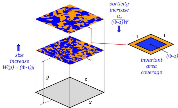
FIG. 10. Two instantaneous wall-parallel slices of the uv product from channel DNS 48 at \delta^+ = 934 . Blue regions denote a negative product, while positive regions are in gold. The average of this quantity, which is negative, constitutes the net wallward flux of momentum. At finite \delta^+ the area coverage of the negative (blue) regions is approximated by \Phi^{-1} = \Phi - 1 , while the average change in scale with increasing y is approximated by (\Phi - 1)y . For the low Reynolds number ( \delta^+ = 934 ) flow depicted, the Fife similarity parameter is about \phi_c = 0.64 , as quantified by the dW^+/dy^+ estimate of figure 6.
