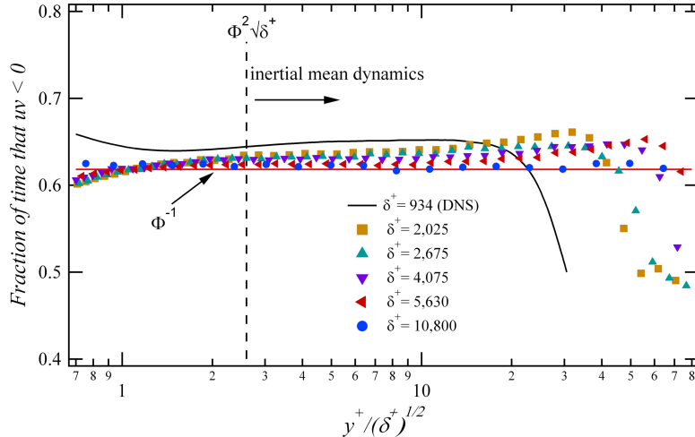
FIG. 7. Area fraction that uv is negative for various \delta^+ and plotted versus y^+/\sqrt{\delta^+} . Data at \delta^+ \simeq 10,800 are from the FPF, while all other measurements are from the HRNBLWT. The line is from channel DNS. 48
