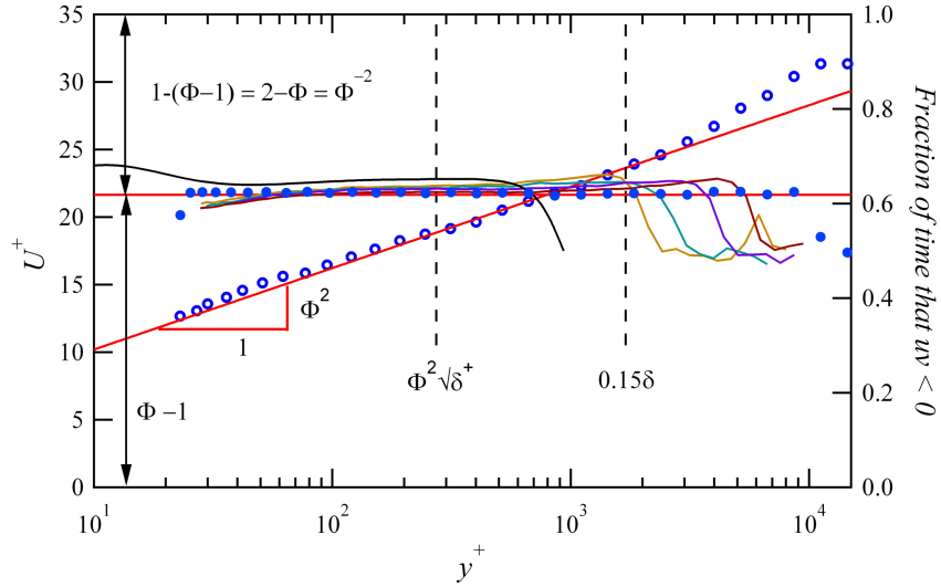
FIG. 9. Logarithmic mean velocity profile at \delta^+ \simeq 10,800 (left axis, open symbols), and area fraction that uv is negative (right axis, lines and solid symbols) versus y^+ . Layers II and III boundaries are indicated for \delta^+ \simeq 10,800 . Lower \delta^+ profiles (lines) are indicated in figure 7.
