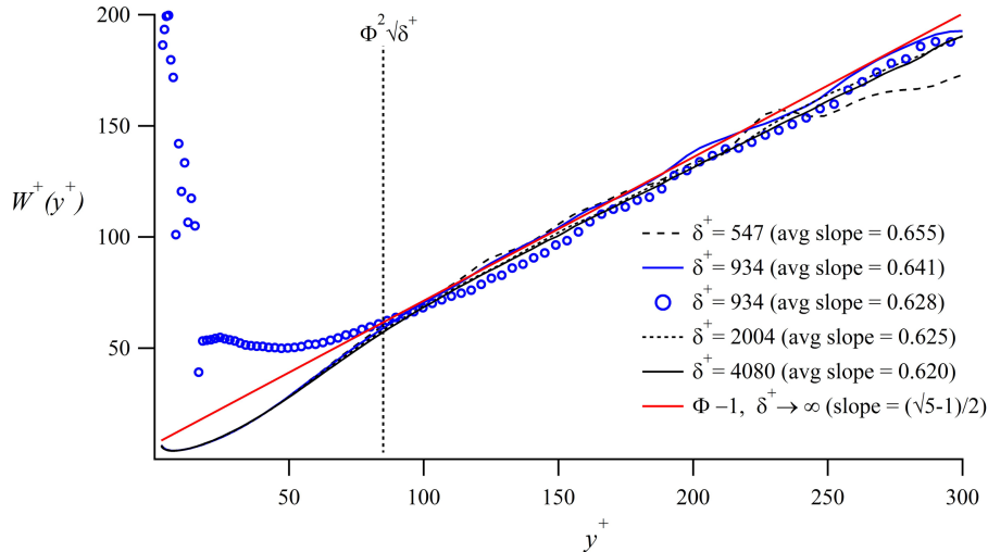
FIG. 6. Length scale distributions, W^+(y^+) , associated with the similarity solution to the mean momentum equation (lines), as compared with the two-dimensional zero-crossing function (circles) determined from planar slices through the instantaneous uv < 0 motions. The vertical line denotes the onset of the inertial domain at \delta^+ = 934 . Data are from channel DNS. 11,43,48
