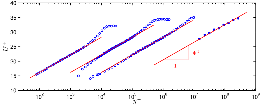
FIG. 5. Semi-logarithmic mean velocity profiles at large \delta^+ reported by Marusic et al. 29 Profiles from left to right are from a wind tunnel boundary layer, water channel boundary layer, pipe flow and atmospheric surface layer. The horizontal axis is shifted by one decade for each respective profile. Red lines denote U^+ = \Phi^2 \ln(y^+) + B . In accord with the analysis of (2), the solid symbols fall within \Phi^2 \sqrt{\delta^+} \lesssim y^+ \lesssim C\delta^+ , where C = 0.15 is employed here.
