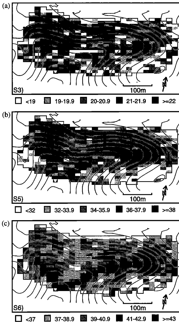
Figure 1. Soil moisture patterns from Tarrawarra showing different degrees of connectivity. (a) random soil moisture pattern February 23, 1996 (S3). (b) developing connectivity April 13, 1996 (S5). (c) connected soil moisture pattern April 22, 1996 (S6). Note that each pixel represents a point measurement of the volumetric soil moisture in the upper 30 cm of the soil profile. Contours show the surface topography; contour intervals are 2 m.
