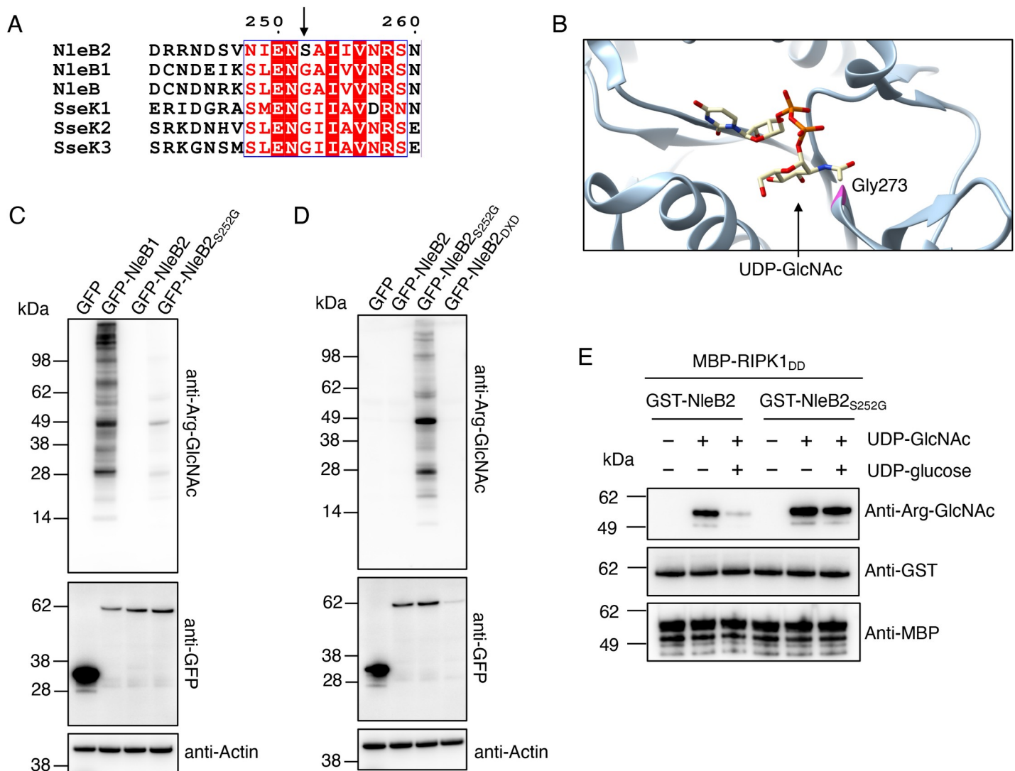
Fig 5. Role of Serine 252 within NleB2 in preference for UDP-glucose. (A) Alignment of NleB2 and NleB1 from EPEC O127:H6 strain E2348/69, NleB from Citrobacter rodentium strain ICC168 and SseK1, SseK2 and SseK3 from Salmonella enterica serovar Typhimurium strain SL1344. Arrow indicates serine 252 within NleB2. Alignment was performed using ClustalW and visualised using ESPript. (B) The crystal structure of SseK2 (PDB ID: 5H63)[18] in complex with UDP-GlcNAc [PMID: 30327479]. The peptide backbone is depicted as a blue ribbon, Glycine 273 is highlighted in pink, and the ligand represented in stick form. The image was generated using Chimera 1.14 with carbon in yellow, nitrogen in blue, oxygen in red and phosphorus in orange. (C) HEK293T cells were transfected with either pEGFP-C2, pGFP-NleB1, pGFP-NleB2 or pGFP-NleB2 S252G before being lysed and subjected to PAGE and immunoblot with anti-Arg-GlcNAc and anti-GFP antibodies. Anti-Actin antibodies were used as a loading control. Representative immunoblots of at least 3 independent experiments. (D) HEK293T cells were transfected with either pEGFP-C2, pGFP-NleB2, pGFP-NleB2 S252G or pGFP-NleB2 DXD before being lysed and subjected to PAGE and immunoblot with anti-Arg-GlcNAc and anti-GFP antibodies. Anti-Actin antibodies were used as a loading control. Representative immunoblots of at least 3 independent experiments. (E) In vitro sugar donor competition assays. MBP-RIPK1 DD was incubated with GST-NleB2 or GST-NleB2 S252G either without sugar donors, or in the presence of 25 \mu M UDP-GlcNAc alone or in combination with 25 \mu M UDP-glucose. Proteins were subjected to PAGE and immunoblot with anti-Arg-GlcNAc, or anti-MBP and anti-GST antibodies as controls. Representative of at least 3 experiments.
